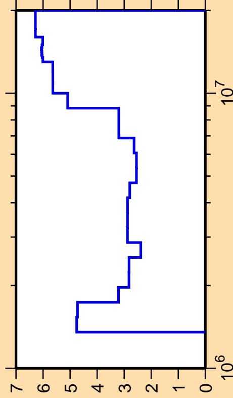
\Delta\sigma/\sigma vs. E for ^{60}\text{Ni}(n,\text{inel.})
