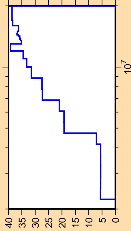
\Delta\sigma/\sigma vs. E for ^{60}\text{Ni}(n,n_3)
