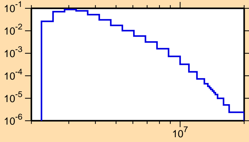
\sigma vs. E for ^{60}\text{Ni}(n,n_3)
