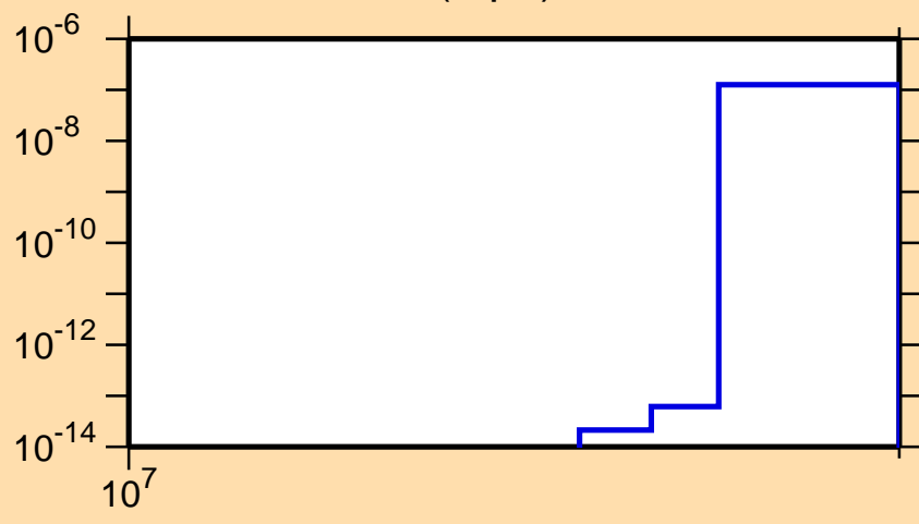
\sigma vs. E for ^{60}\text{Ni}(n,\text{pd})
