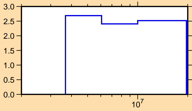
\Delta\sigma/\sigma vs. E for ^{60}\text{Ni}(n,n\text{nonel.})
