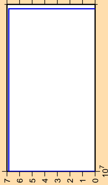
\Delta\sigma/\sigma vs. E for ^{60}\text{Ni}(n,n\text{cont.})
