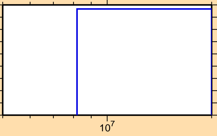
\sigma vs. E for ^{60}\text{Ni}(n,\text{nd})
