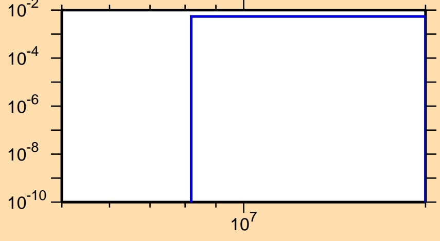
\sigma vs. E for ^{60}\text{Ni}(n,n\alpha)
