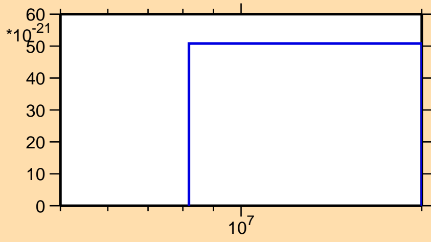
\sigma vs. E for ^{60}\text{Ni} (mt 34)
