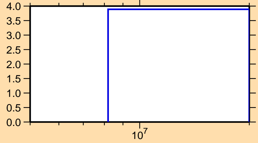
\Delta\sigma/\sigma vs. E for ^{62}\text{Ni}(n,2n)
