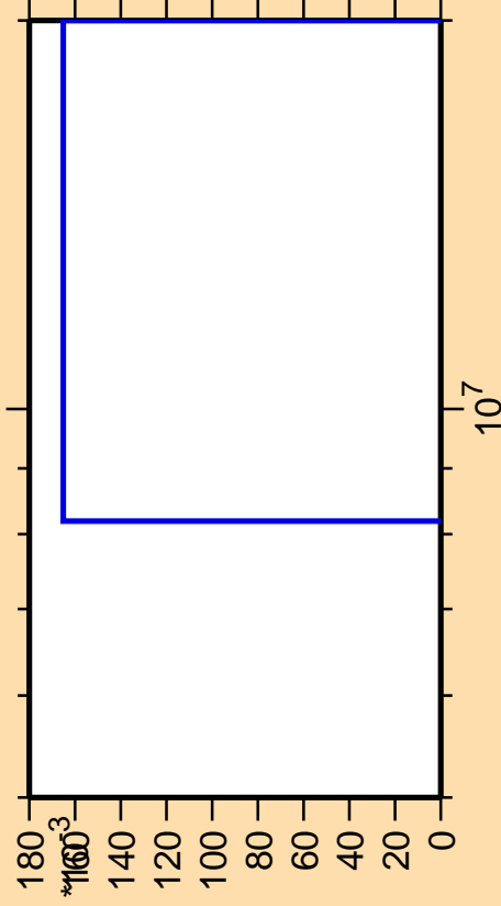
\Delta\sigma/\sigma vs. E for ^{62}\text{Ni}(n,\text{nd})
