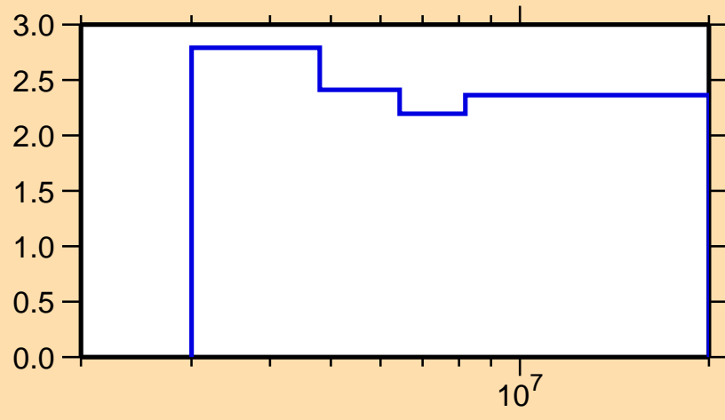
\Delta\sigma/\sigma vs. E for ^{62}\text{Ni}(n,n\text{nonel.})
