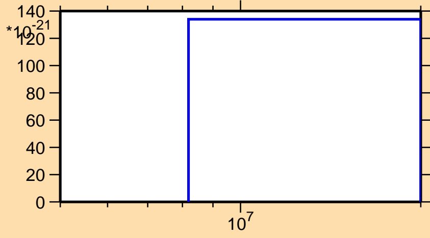
\sigma vs. E for ^{63}\text{Ni}(\text{mt } 34)
