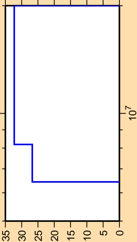
\Delta\sigma/\sigma vs. E for ^{63}\text{Ni}(n,\gamma)
