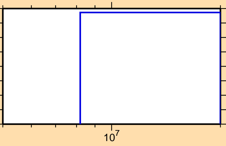
\sigma vs. E for ^{63}\text{Ni}(n,np)
