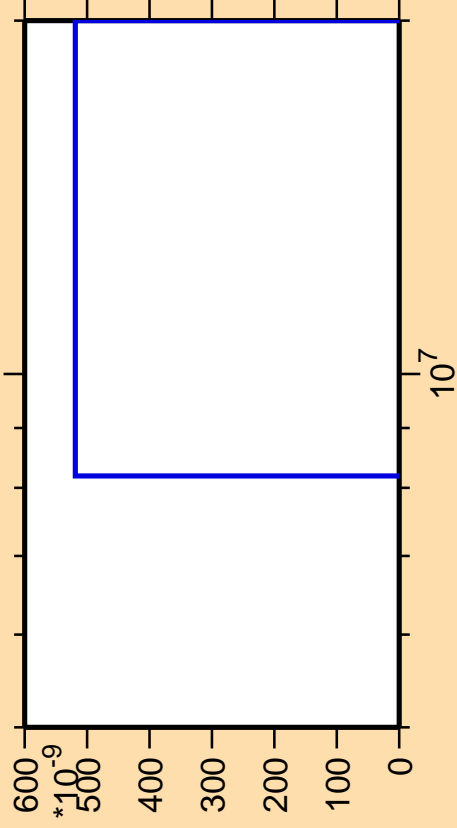
\Delta\sigma/\sigma vs. E for ^{63}\text{Ni}(\text{mt } 34)
