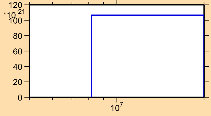
\sigma vs. E for ^{63}\text{Ni}(n,\text{nt})
