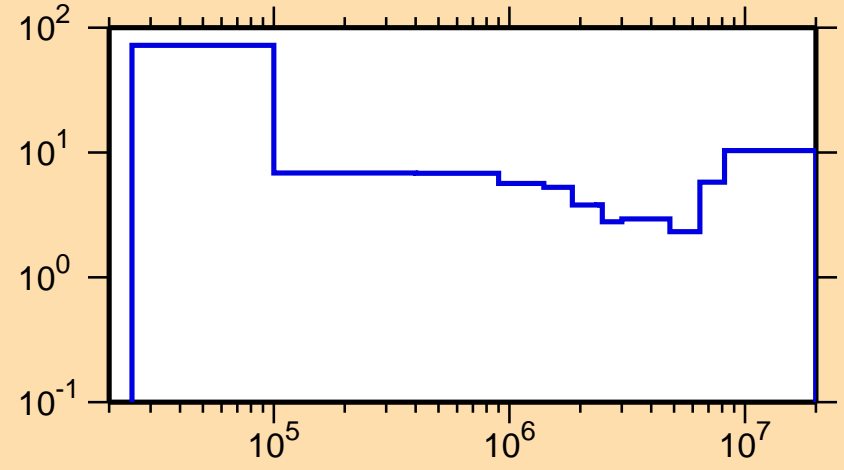
\Delta\sigma/\sigma vs. E for ^{63}\text{Ni}(n,\text{inel.})
