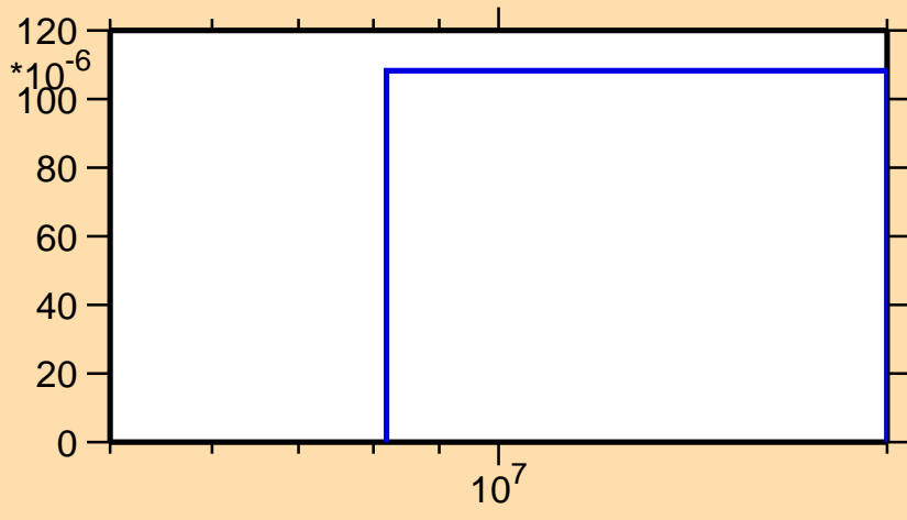
\sigma vs. E for ^{63}\text{Ni}(n,t)
