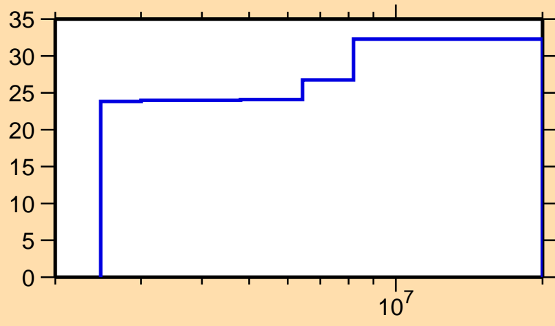
\Delta\sigma/\sigma vs. E for ^{63}\text{Ni}(n,\gamma)
