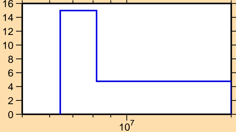
\Delta\sigma/\sigma vs. E for ^{63}\text{Ni}(n,2n)
