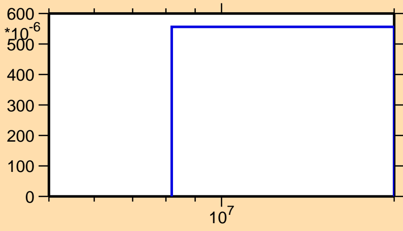
\sigma vs. E for ^{63}\text{Ni}(n,n\alpha)
