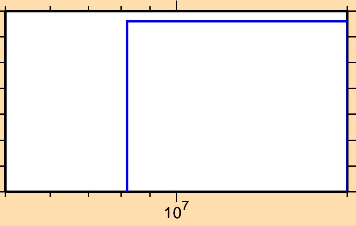
\sigma vs. E for ^{63}\text{Ni}(n,\text{nd})
