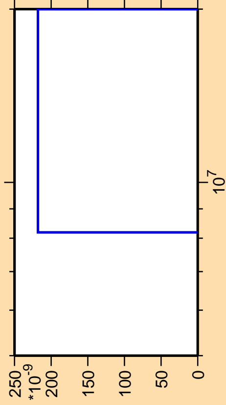
\Delta\sigma/\sigma vs. E for ^{63}\text{Ni}(n,\text{nt})
