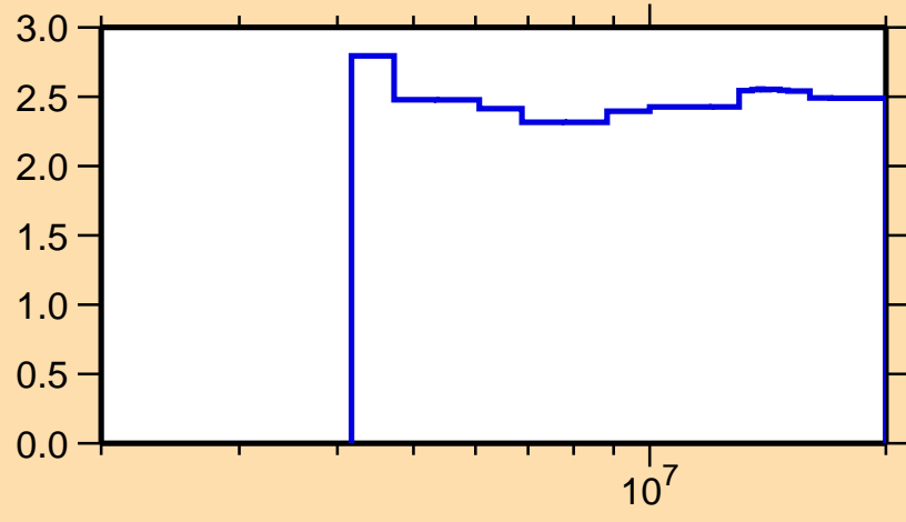
\Delta\sigma/\sigma vs. E for ^{64}\text{Ni}(n,n\text{onel.})
