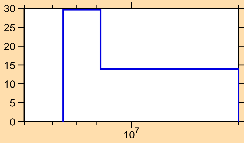
\Delta\sigma/\sigma vs. E for ^{64}\text{Ni}(n,p)
