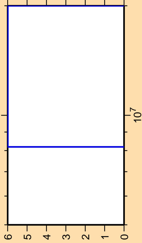
\Delta\sigma/\sigma vs. E for ^{64}\text{Ni}(n,2n)
