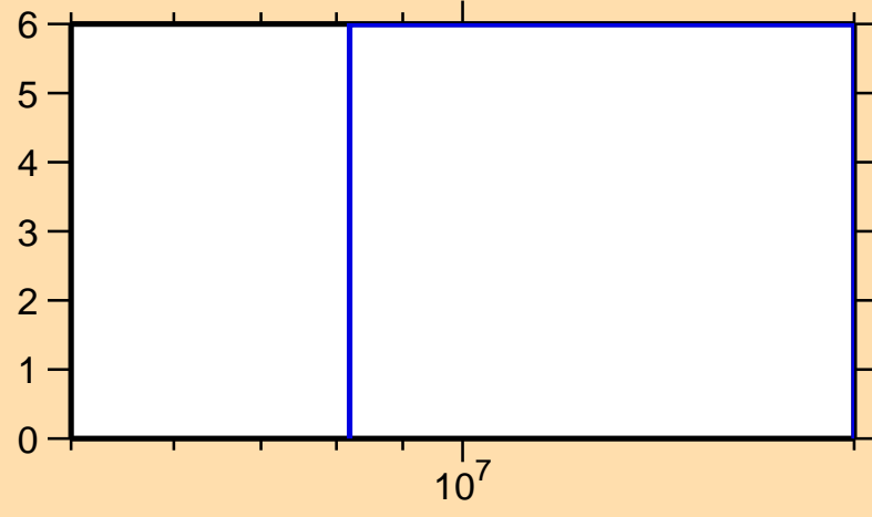
\Delta\sigma/\sigma vs. E for ^{64}\text{Ni}(n,2n)
