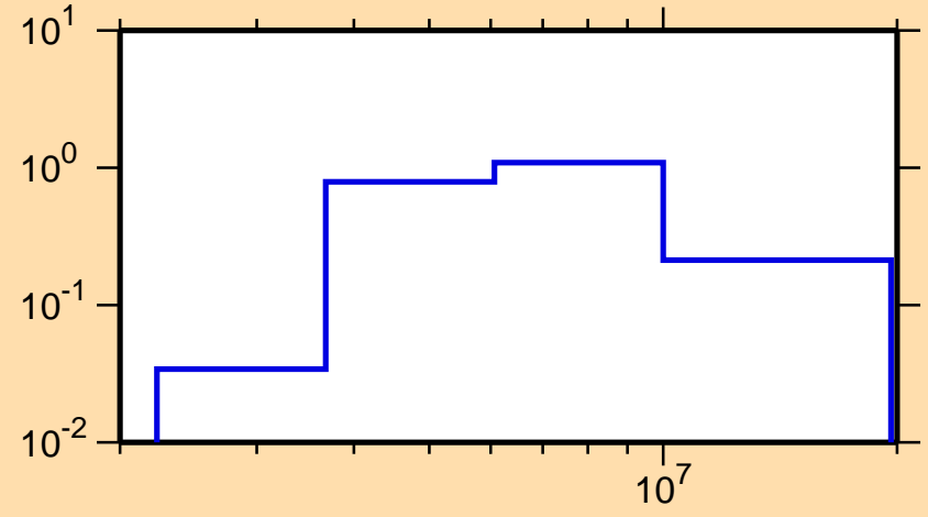
\sigma vs. E for ^{65}\text{Ni}(n,n\text{cont.})
