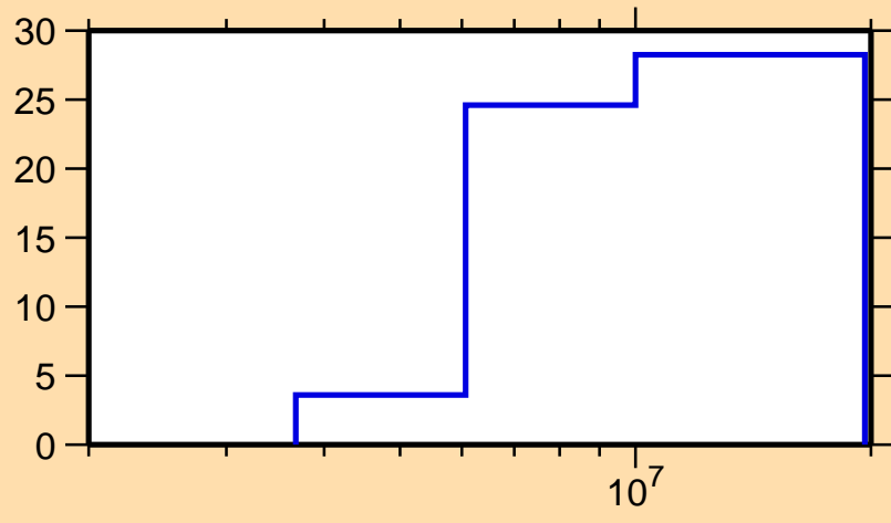
\Delta\sigma/\sigma vs. E for ^{65}\text{Ni}(n,p)
