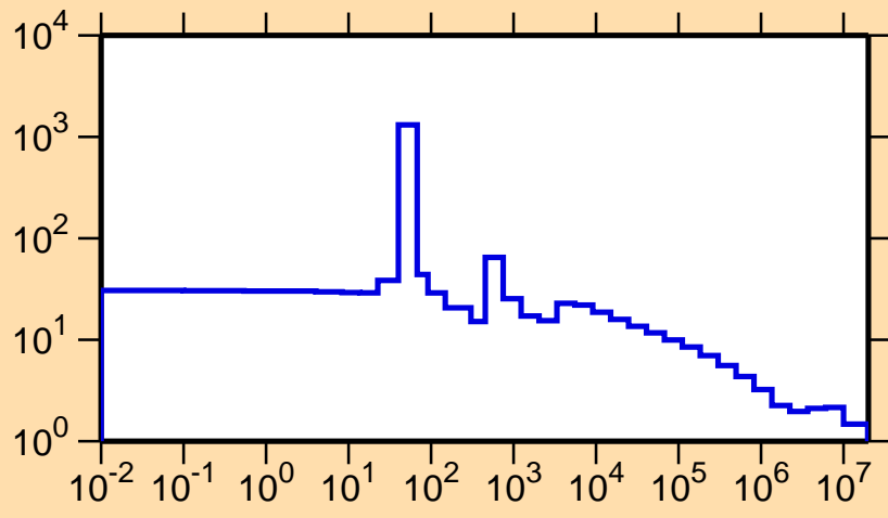
\sigma vs. E for ^{65}\text{Ni}(n,\text{el.})
