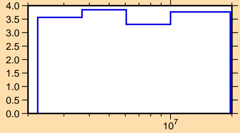
\Delta\sigma/\sigma vs. E for ^{65}\text{Ni}(n,\text{nonel.})
