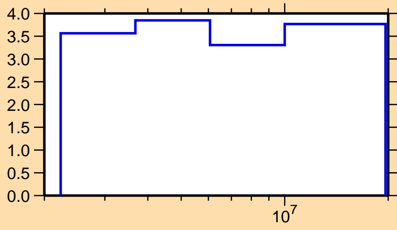
\Delta\sigma/\sigma vs. E for ^{65}\text{Ni}(n,n\text{onel.})
