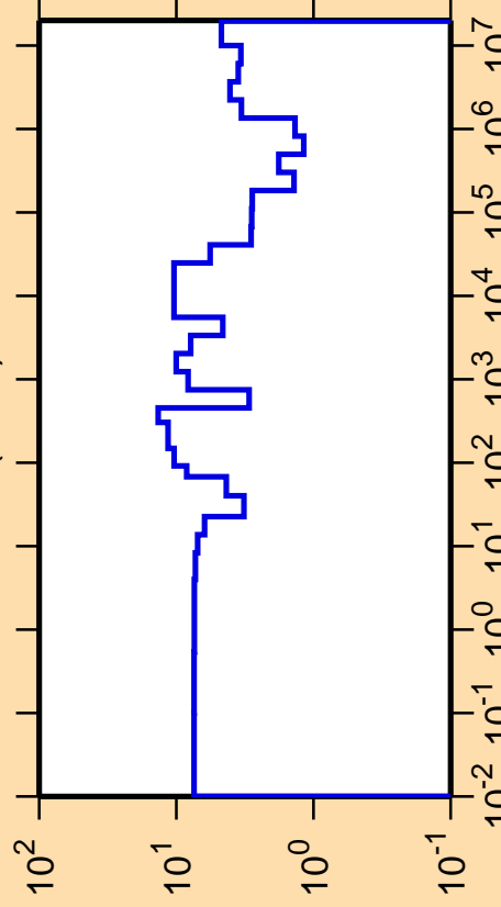
\Delta\sigma/\sigma vs. E for ^{65}\text{Ni}(n,\text{el.})
