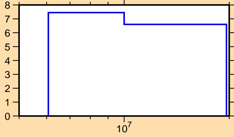
\Delta\sigma/\sigma vs. E for ^{65}\text{Ni}(n,2n)
