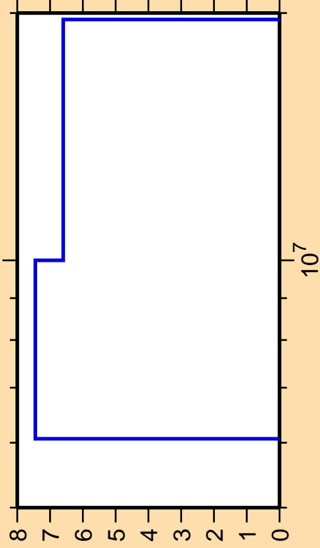
\Delta\sigma/\sigma vs. E for ^{65}\text{Ni}(n,2n)
