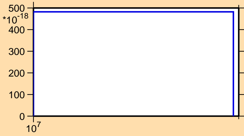
\sigma vs. E for ^{66}\text{Ni}(n,nt)
