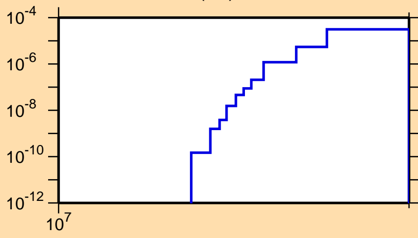
\sigma vs. E for ^{67}\text{Ni}(n,t)
