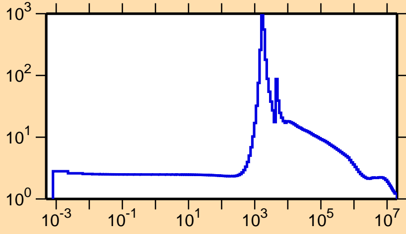
\sigma vs. E for ^{67}\text{Ni}(n,\text{el.})
