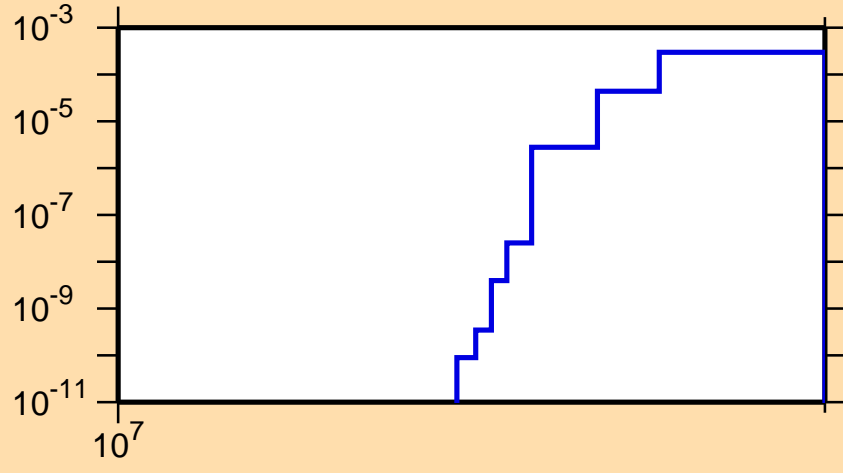
\sigma vs. E for ^{67}\text{Ni}(n,d)
