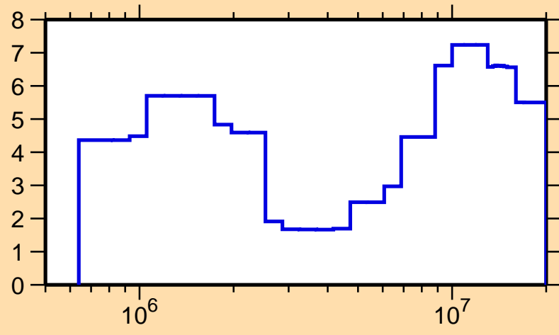
\Delta\sigma/\sigma vs. E for ^{67}\text{Ni}(n,\text{tot.})
