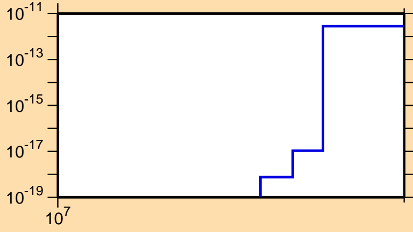
\sigma vs. E for ^{67}\text{Ni}(n,2n\alpha)
