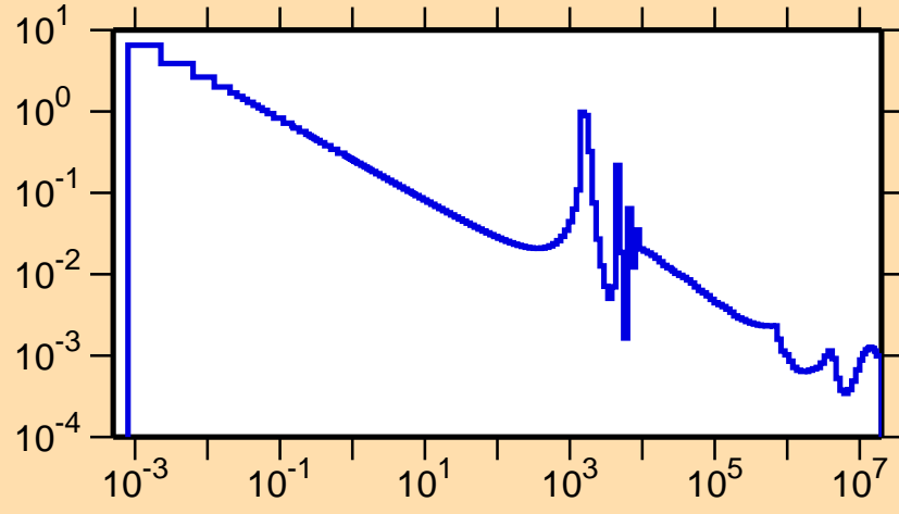
\sigma vs. E for ^{67}\text{Ni}(n,\gamma)
