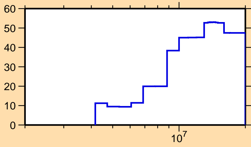
\Delta\sigma/\sigma vs. E for ^{67}\text{Ni}(n,n\text{cont.})
