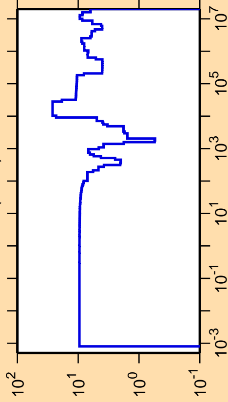
\Delta\sigma/\sigma vs. E for ^{67}\text{Ni}(n,\text{el.})
