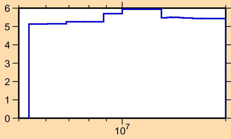
\Delta\sigma/\sigma vs. E for ^{67}\text{Ni}(n,\text{nonel.})
