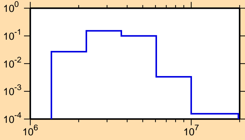
\sigma vs. E for ^{67}\text{Ni}(n,n_4)
