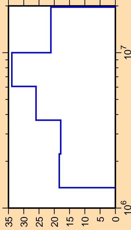
\Delta\sigma/\sigma vs. E for ^{67}\text{Ni}(n,n_4)
