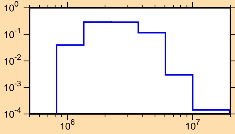
\sigma vs. E for ^{67}\text{Ni}(n,n_3)
