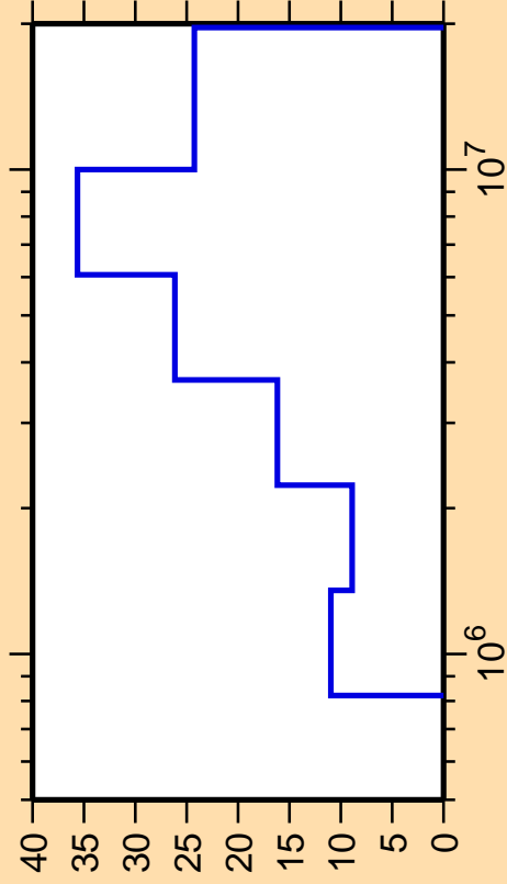
\Delta\sigma/\sigma vs. E for ^{67}\text{Ni}(n,n_3)
