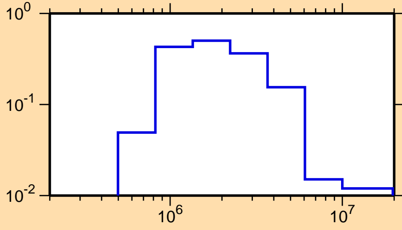
\sigma vs. E for ^{67}\text{Ni}(n,n_1)
