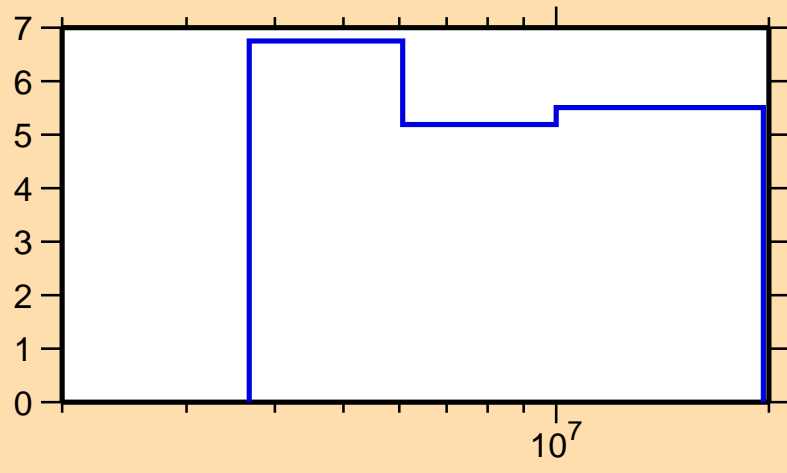
\Delta\sigma/\sigma vs. E for ^{67}\text{Ni}(n,n\text{nonel.})
