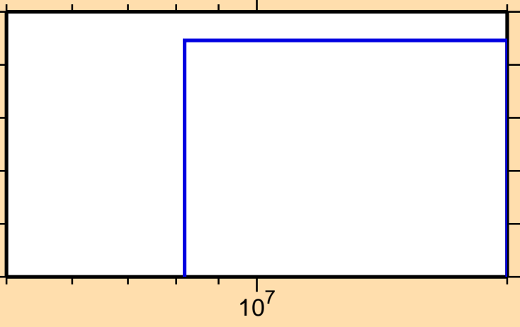
\sigma vs. E for ^{67}\text{Ni}(n,d)
