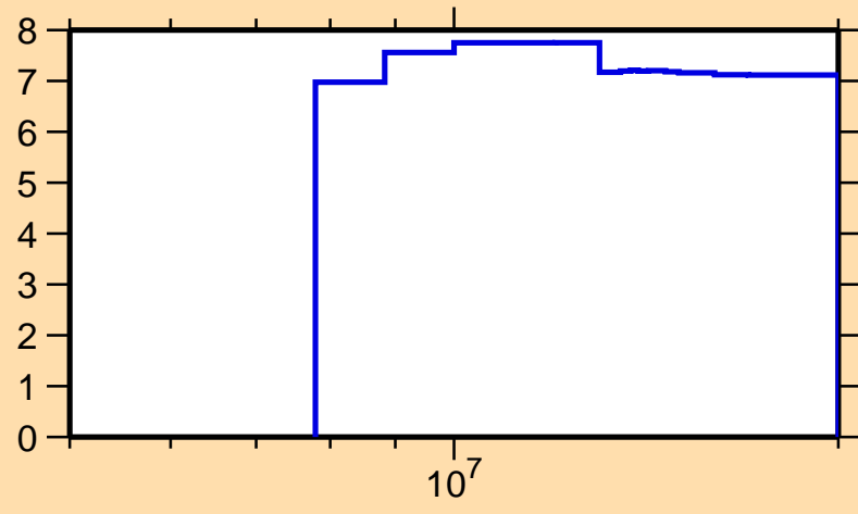
\Delta\sigma/\sigma vs. E for ^{68}\text{Ni}(n,\text{nonel.})
