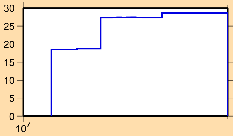
\Delta\sigma/\sigma vs. E for ^{68}\text{Ni}(n,ncont.)
