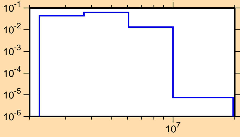
\sigma vs. E for ^{68}\text{Ni}(n,n_3)
