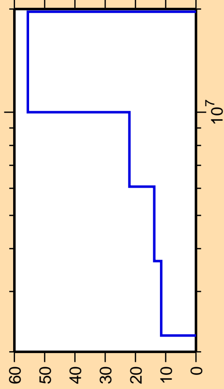
\Delta\sigma/\sigma vs. E for ^{68}\text{Ni}(n,n_4)
