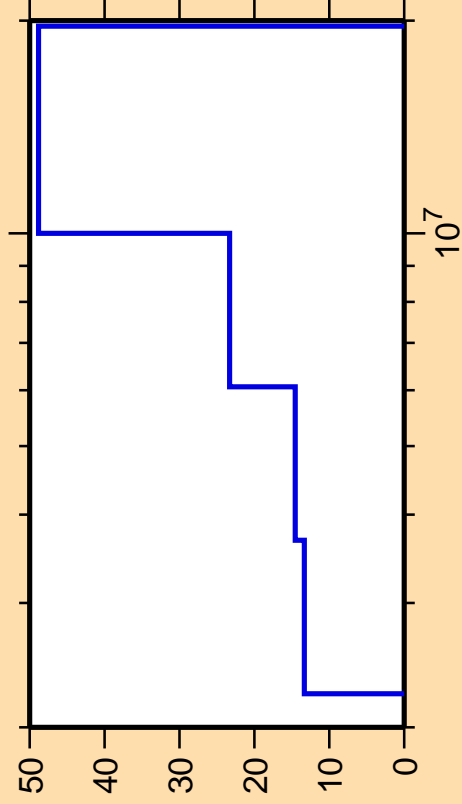
\Delta\sigma/\sigma vs. E for ^{68}\text{Ni}(n,n_3)
