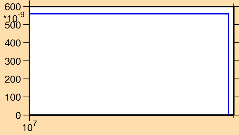
\sigma vs. E for ^{69}\text{Ni}(n,d)
