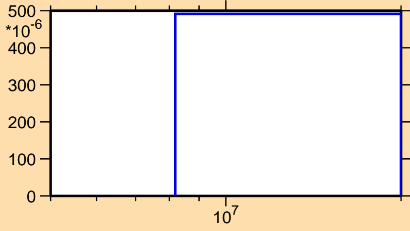
\sigma vs. E for ^{69}\text{Ni}(n,p)
