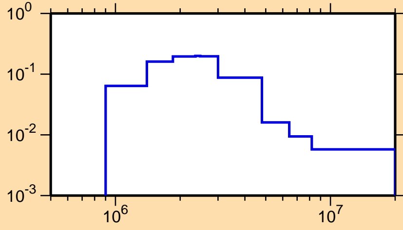
\sigma vs. E for ^{69}\text{Ni}(n,n_2)
