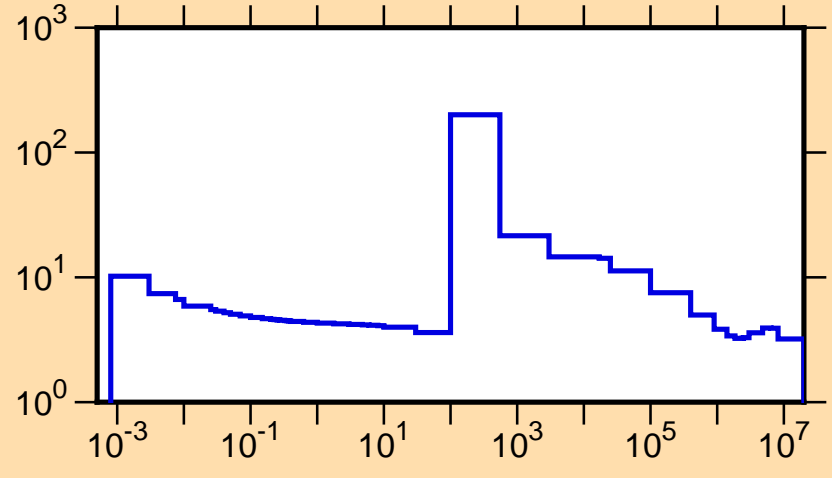
\sigma vs. E for ^{69}\text{Ni}(n,\text{tot.})
