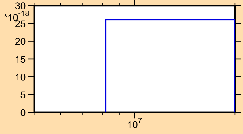
\sigma vs. E for ^{69}\text{Ni}(n,nt)
