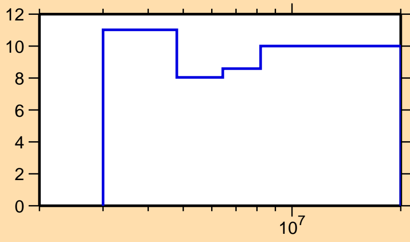
\Delta\sigma/\sigma vs. E for ^{69}\text{Ni}(n,n\text{nonel.})
