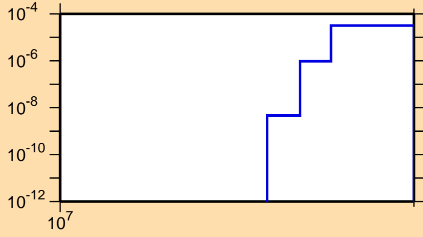
\sigma vs. E for ^{70}\text{Ni}(n,d)
