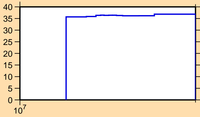
\Delta\sigma/\sigma vs. E for ^{70}\text{Ni}(n,n_1)
