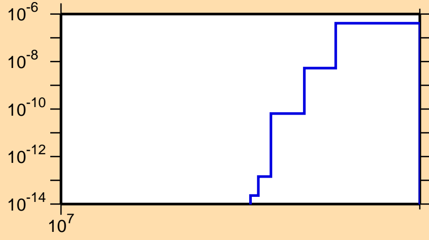
\sigma vs. E for ^{70}\text{Ni}(n,n\alpha)
