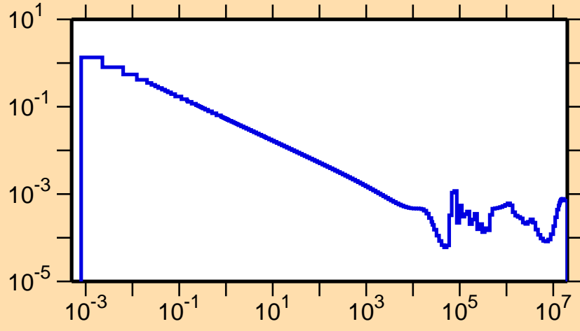
\sigma vs. E for ^{70}\text{Ni}(n,\gamma)
