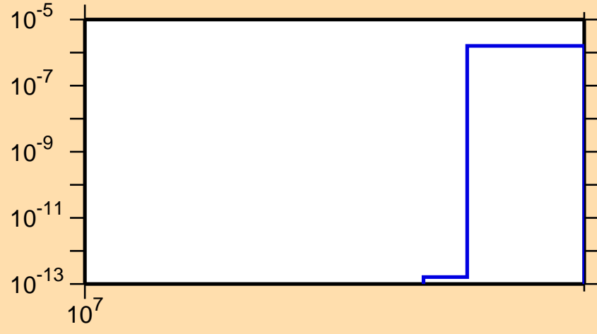
\sigma vs. E for ^{70}\text{Ni}(n,np)
