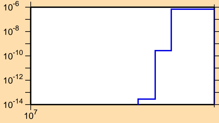
\sigma vs. E for ^{70}\text{Ni}(n,t)
