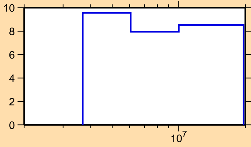
\Delta\sigma/\sigma vs. E for ^{70}\text{Ni}(n,n\text{nonel.})
