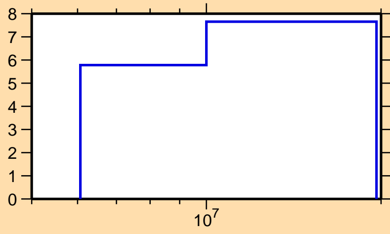
\Delta\sigma/\sigma vs. E for ^{70}\text{Ni}(n,\text{tot.})
