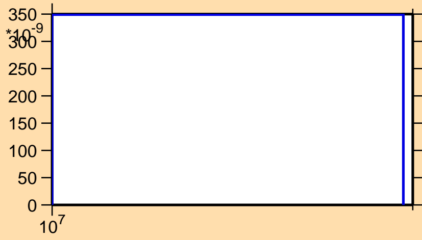
\sigma vs. E for ^{70}\text{Ni}(n,d)
