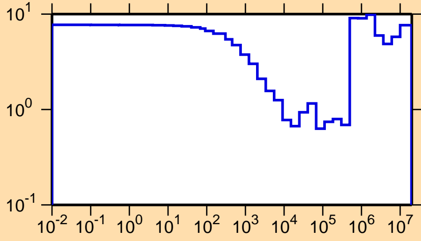
\Delta\sigma/\sigma vs. E for ^{70}\text{Ni}(n,\text{tot.})
