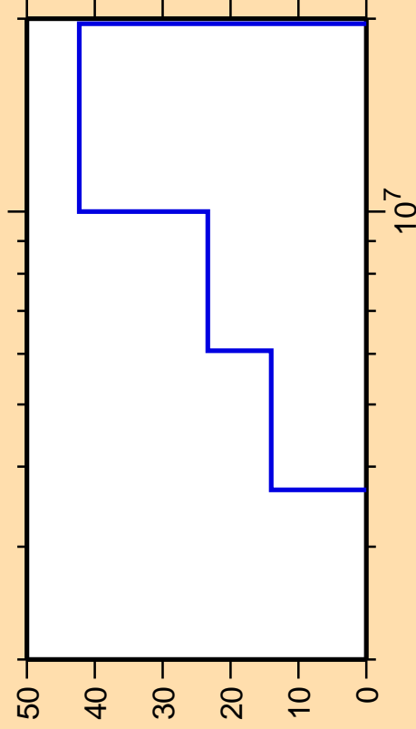
\Delta\sigma/\sigma vs. E for ^{70}\text{Ni}(n,n\text{cont.})
