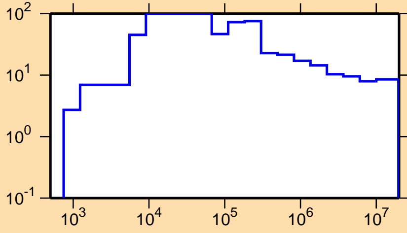
\Delta\sigma/\sigma vs. E for ^{70}\text{Ni}(n,\text{nonel.})
