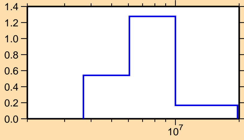
\sigma vs. E for ^{70}\text{Ni}(n,n\text{cont.})
