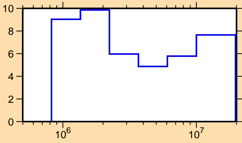
\Delta\sigma/\sigma vs. E for ^{70}\text{Ni}(n,\text{tot.})
