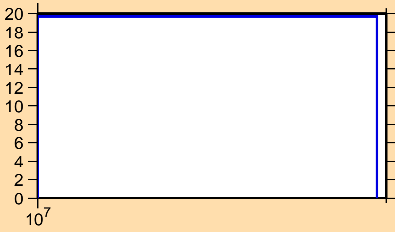
\Delta\sigma/\sigma vs. E for ^{70}\text{Ni}(n,2n)
