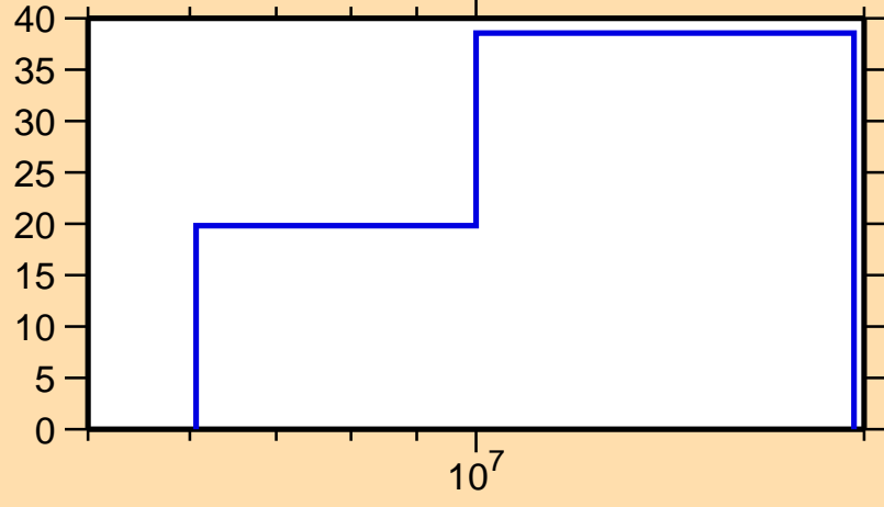
\Delta\sigma/\sigma vs. E for ^{70}\text{Ni}(n,\text{inel.})
