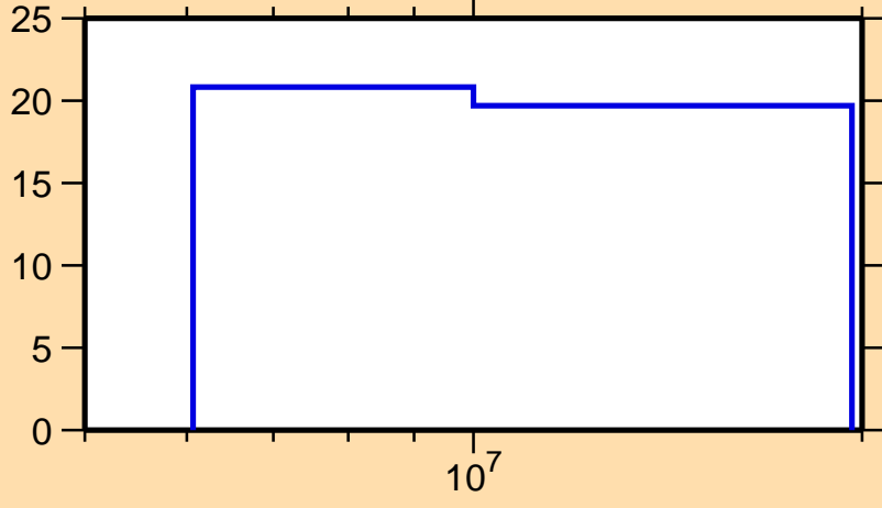
\Delta\sigma/\sigma vs. E for ^{70}\text{Ni}(n,2n)
