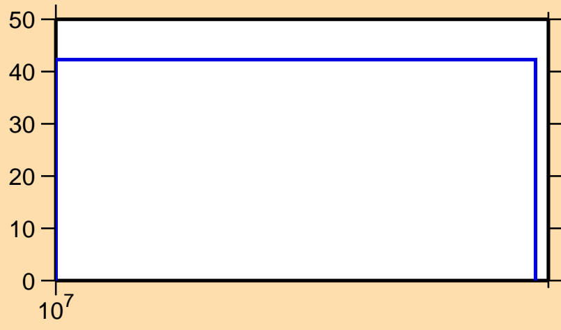
\Delta\sigma/\sigma vs. E for ^{70}\text{Ni}(n,n\text{cont.})
