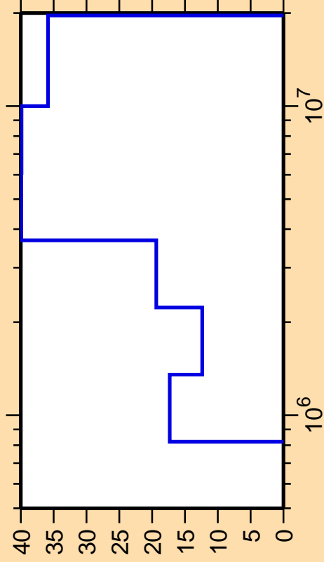
\Delta\sigma/\sigma vs. E for ^{70}\text{Ni}(n,n_1)
