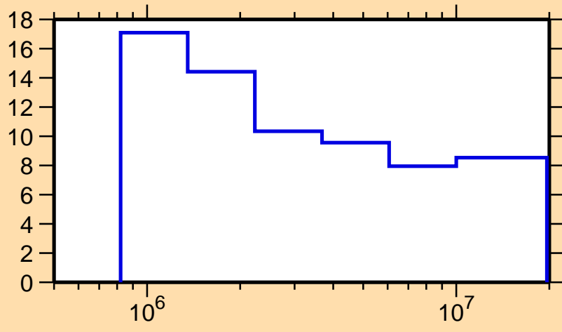
\Delta\sigma/\sigma vs. E for ^{70}\text{Ni}(n,\text{nonel.})
