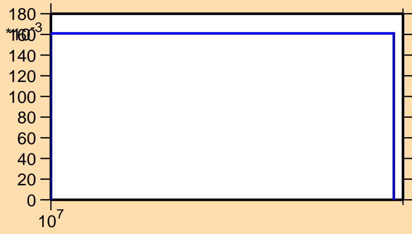
\sigma vs. E for ^{70}\text{Ni}(n,3n)
