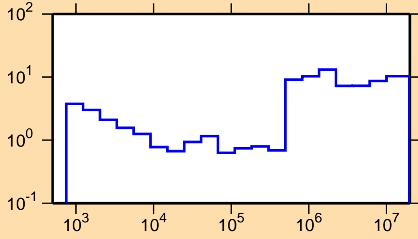
\Delta\sigma/\sigma vs. E for ^{70}\text{Ni}(n,\text{el.})
