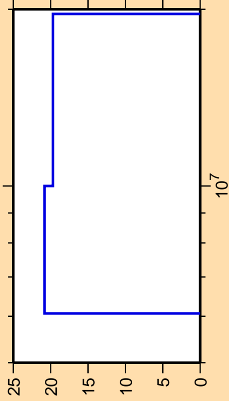
\Delta\sigma/\sigma vs. E for ^{70}\text{Ni}(n,2n)
