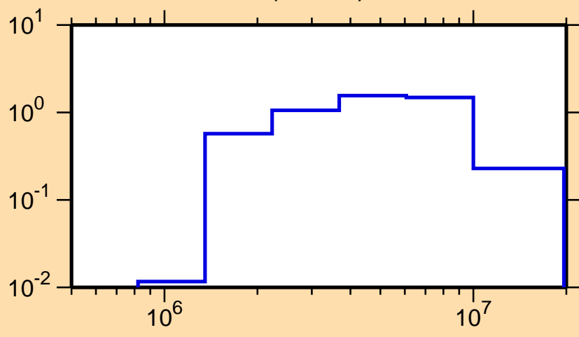
\sigma vs. E for ^{70}\text{Ni}(n,\text{inel.})
