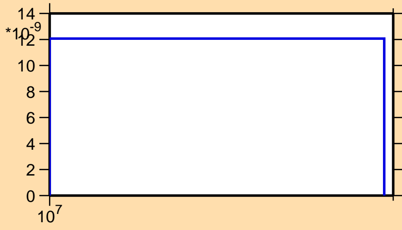
\sigma vs. E for ^{70}\text{Ni}(n,np)
