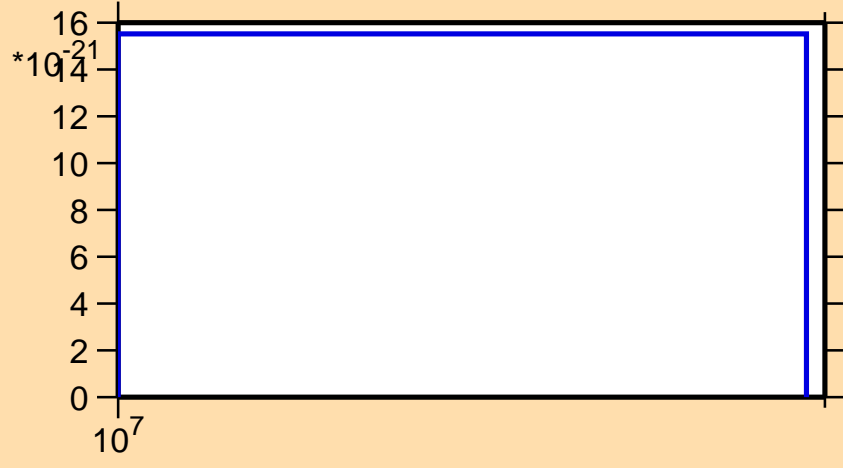
\sigma vs. E for ^{70}\text{Ni}(n,nt)
