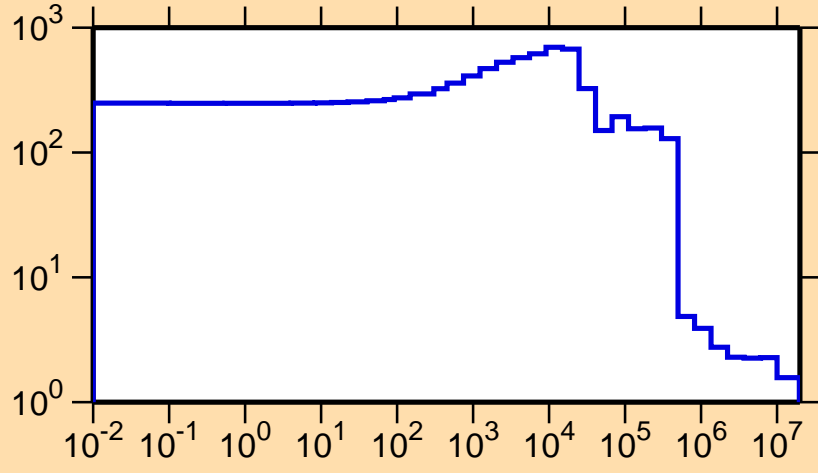
\sigma vs. E for ^{70}\text{Ni}(n,\text{el.})
