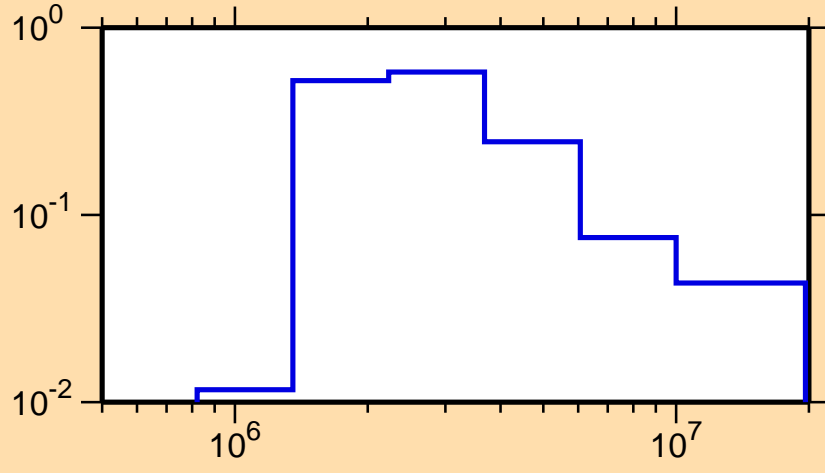
\sigma vs. E for ^{70}\text{Ni}(n,n_1)
