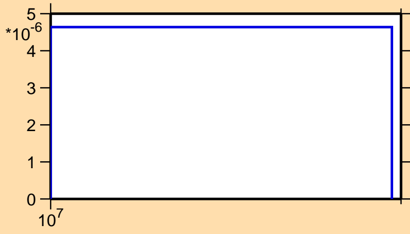
\sigma vs. E for ^{70}\text{Ni}(n,p)
