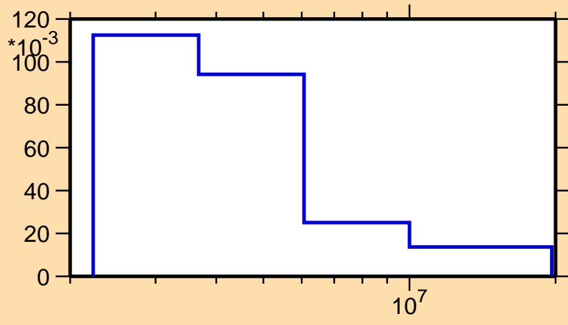
\sigma vs. E for ^{70}\text{Ni}(n,n_3)
