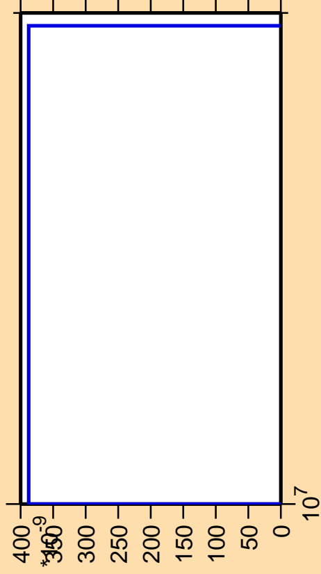
\Delta\sigma/\sigma vs. E for ^{70}\text{Ni}(n,nt)
