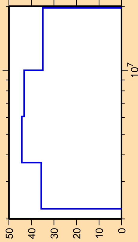
\Delta\sigma/\sigma vs. E for ^{70}\text{Ni}(n,n_3)
