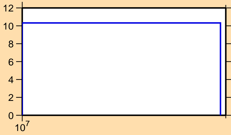
\Delta\sigma/\sigma vs. E for ^{70}\text{Ni}(n,\text{el.})
