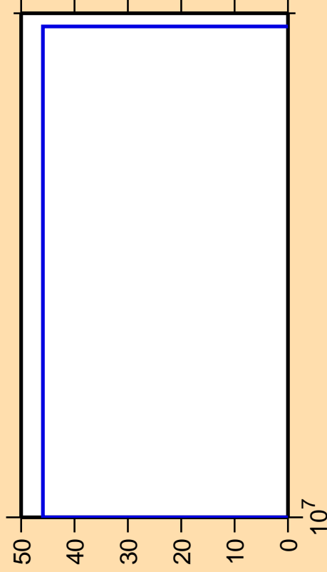
\Delta\sigma/\sigma vs. E for ^{70}\text{Ni}(n,d)
