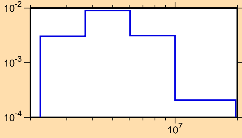
\sigma vs. E for ^{70}\text{Ni}(n,n_4)
