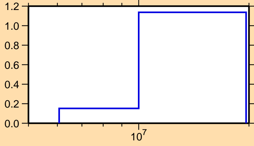
\sigma vs. E for ^{70}\text{Ni}(n,2n)
