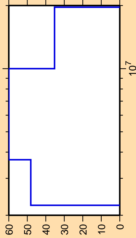
\Delta\sigma/\sigma vs. E for ^{70}\text{Ni}(n,n_4)
