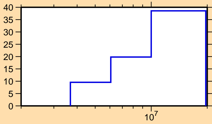
\Delta\sigma/\sigma vs. E for ^{70}\text{Ni}(n,\text{inel.})
