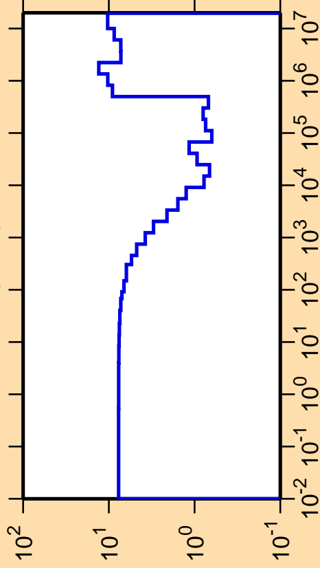
\Delta\sigma/\sigma vs. E for ^{70}\text{Ni}(n,\text{el.})
