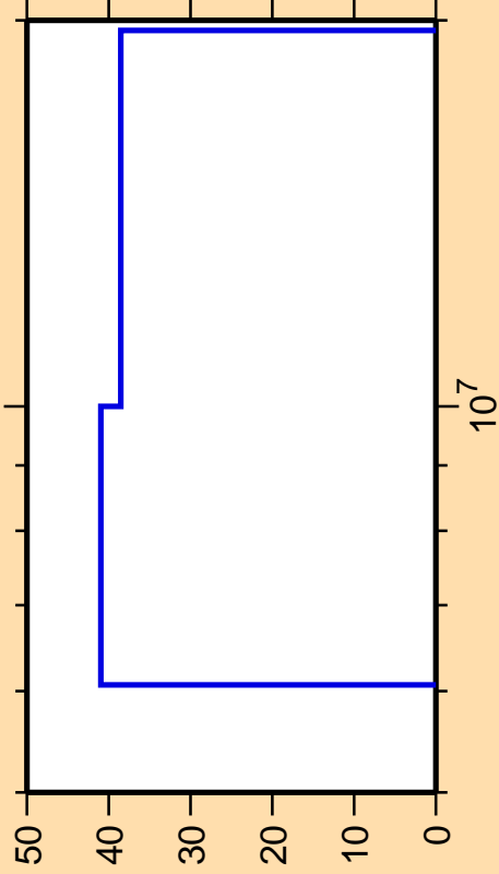
\Delta\sigma/\sigma vs. E for ^{70}\text{Ni}(n,\gamma)
