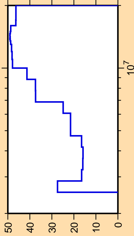
\Delta\sigma/\sigma vs. E for ^{71}\text{Ni}(n,\text{ncont.})
