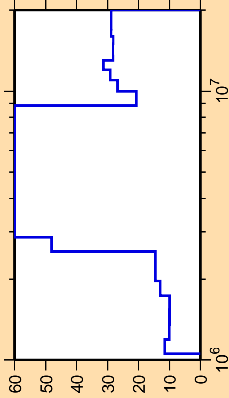
\Delta\sigma/\sigma vs. E for ^{71}\text{Ni}(n,n_4)
