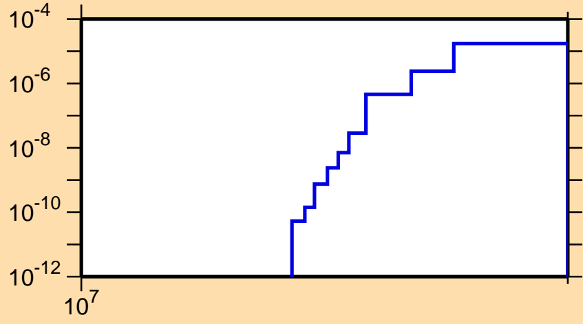
\sigma vs. E for ^{71}\text{Ni}(n,t)
