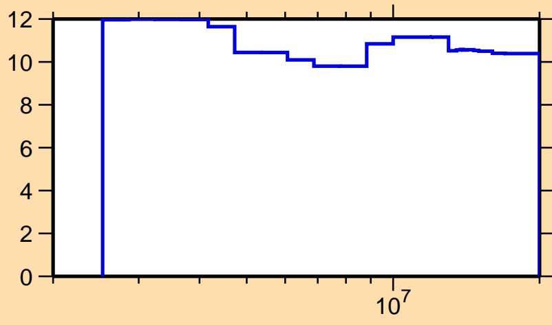
\Delta\sigma/\sigma vs. E for ^{71}\text{Ni}(n,n\text{onel.})
