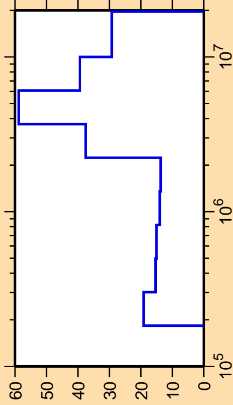
\Delta\sigma/\sigma vs. E for ^{71}\text{Ni}(n,n_1)
