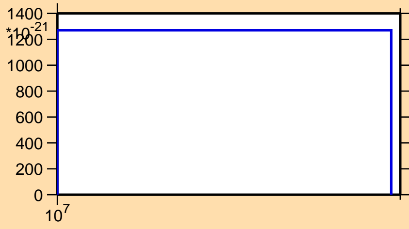
\sigma vs. E for ^{71}\text{Ni}(n,nt)
