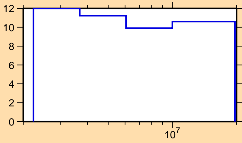
\Delta\sigma/\sigma vs. E for ^{71}\text{Ni}(n,n\text{nonel.})
