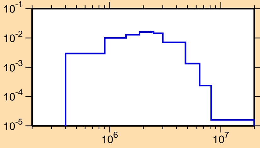
\sigma vs. E for ^{71}\text{Ni}(n,n_2)
