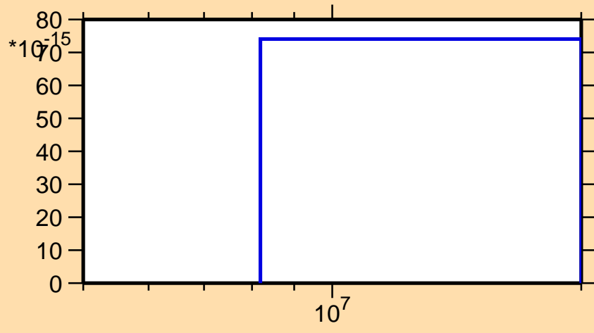
\sigma vs. E for ^{71}\text{Ni}(n,\text{nd})
