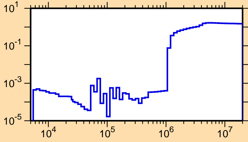
\sigma vs. E for ^{72}\text{Ni}(n,\text{nonel.})
