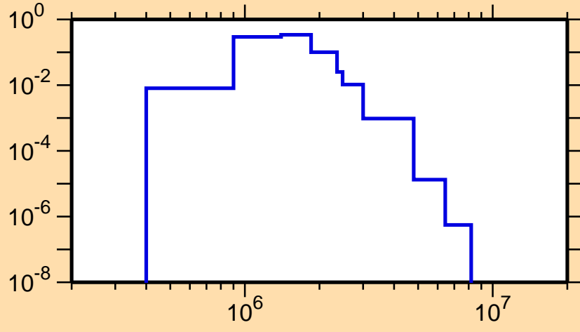
\sigma vs. E for ^{251}\text{No}(n,n_4)
