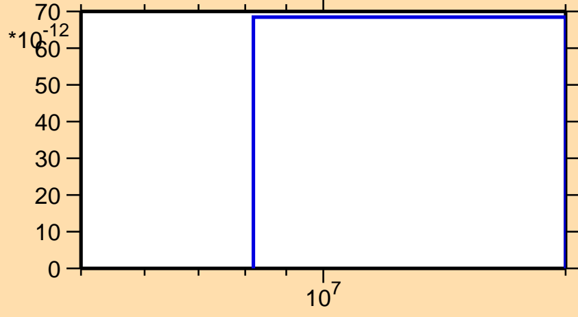
\sigma vs. E for ^{251}\text{No}(n,\text{nd})
