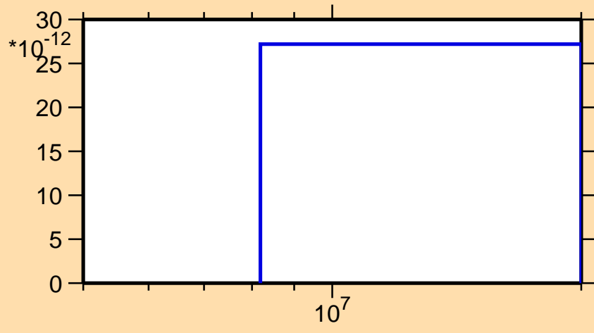
\sigma vs. E for ^{251}\text{No}(\text{mt } 45)
