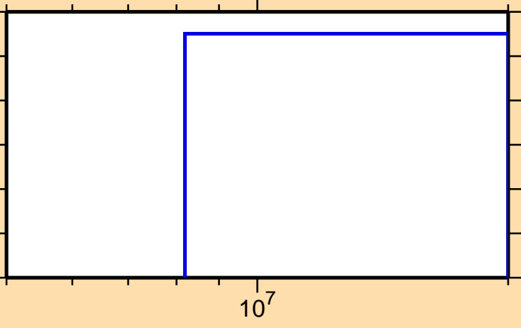
\sigma vs. E for ^{252}\text{No}(n,\text{pd})
