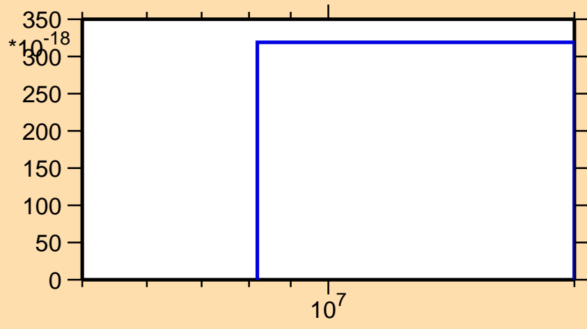
\sigma vs. E for ^{252}\text{No}(\text{mt } 34)
