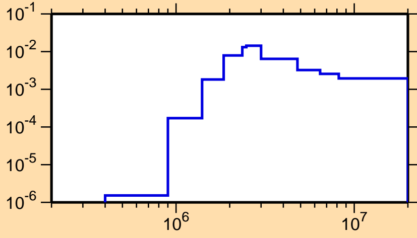
\sigma vs. E for ^{252}\text{No}(n,n_4)
