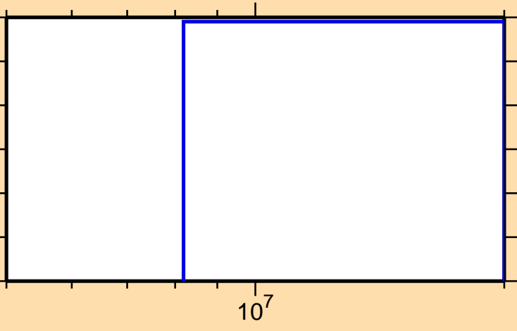
\sigma vs. E for ^{252}\text{No}(n,\text{nd})
