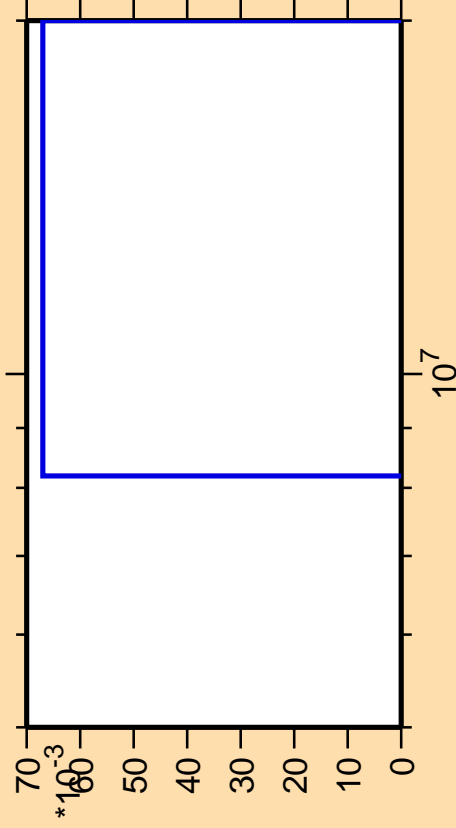
\Delta\sigma/\sigma vs. E for ^{252}\text{No}(\text{mt117})
