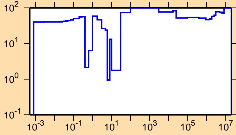
\Delta\sigma/\sigma vs. E for ^{252}\text{No}(n,\gamma)
