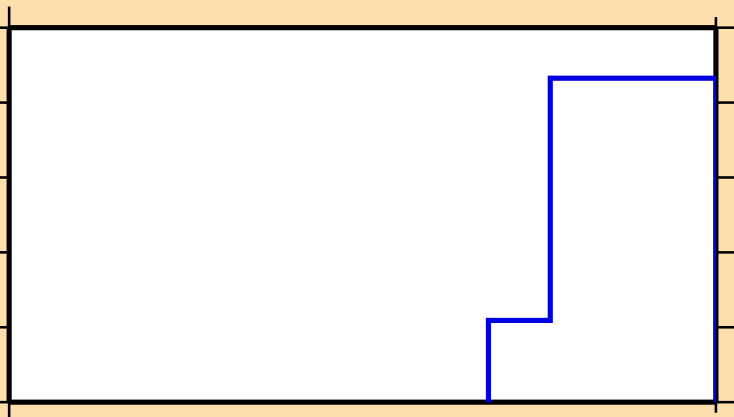
\sigma vs. E for ^{253}\text{No}(\text{mt117})
