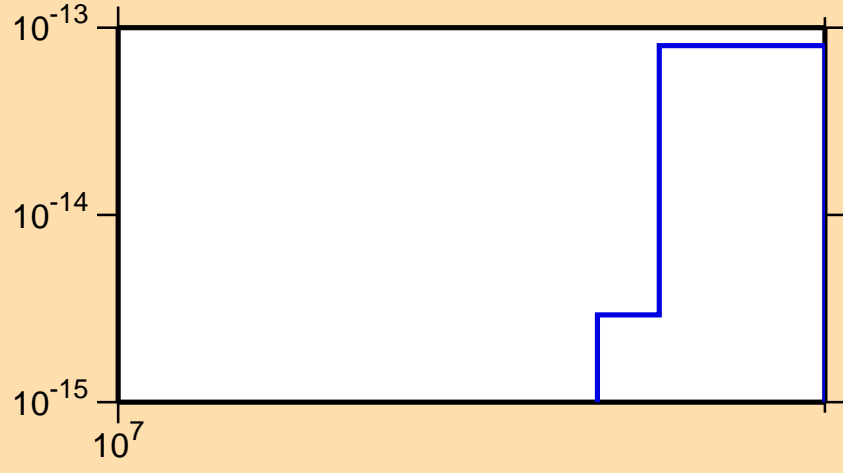
\sigma vs. E for ^{253}\text{No}(n,\text{pt})
