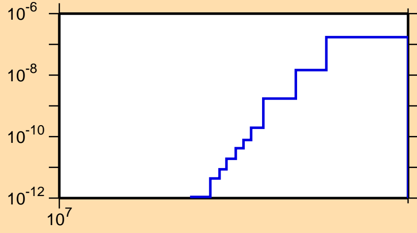
\sigma vs. E for ^{253}\text{No}(n,\text{nd})
