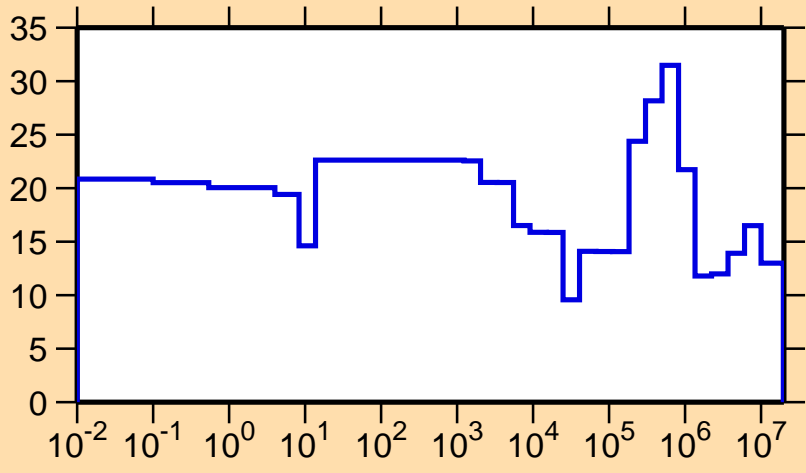
\Delta\sigma/\sigma vs. E for ^{253}\text{No}(n,el.)
