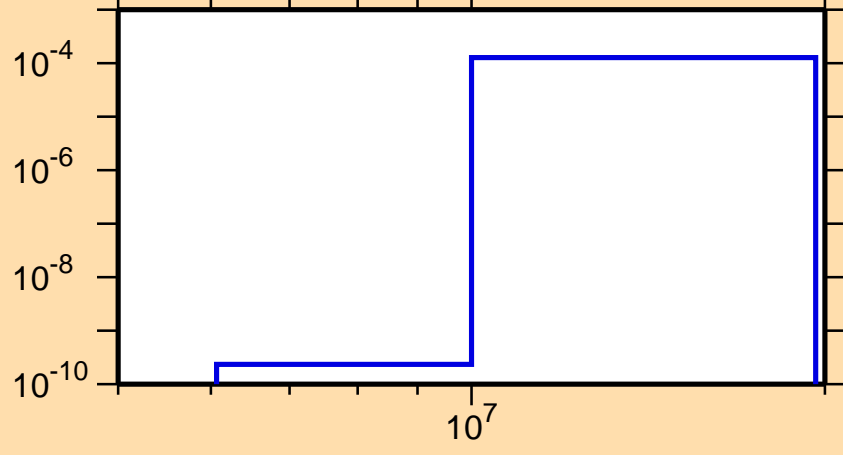
\sigma vs. E for ^{253}\text{No}(n,t)
