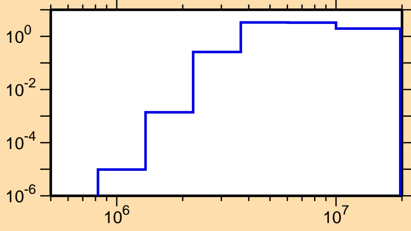
\sigma vs. E for ^{253}\text{No}(n,n\text{cont.})
