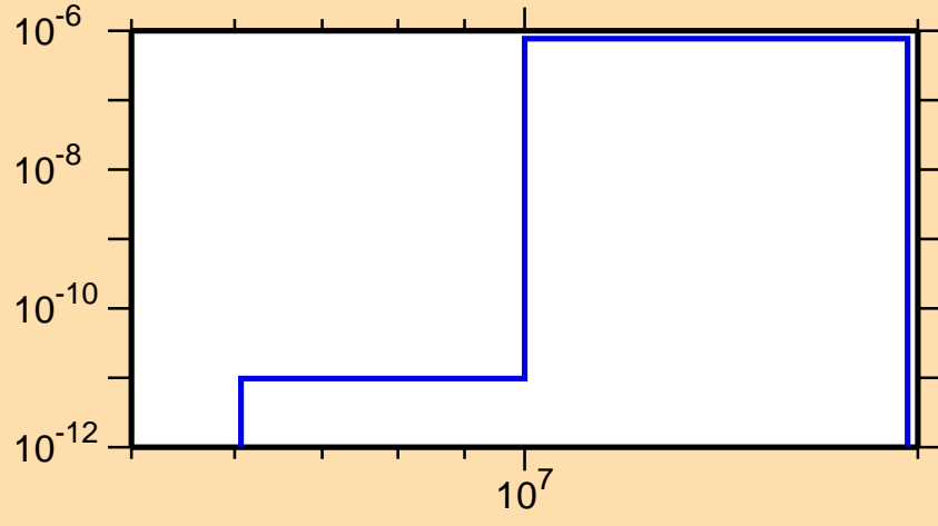
\sigma vs. E for ^{253}\text{No}(n,2n\alpha)
