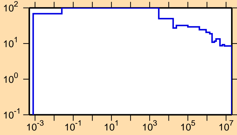
\Delta\sigma/\sigma vs. E for ^{253}\text{No}(n,\text{nonel.})
