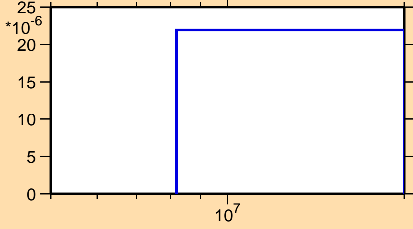
\sigma vs. E for ^{253}\text{No}(n,3n)
