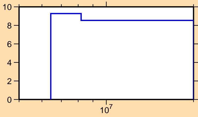
\Delta\sigma/\sigma vs. E for ^{253}\text{No}(n,\text{nonel.})
