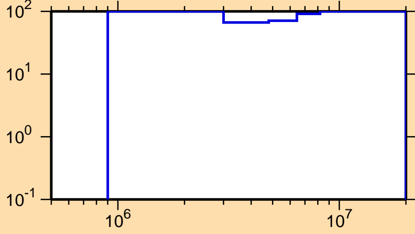
\Delta\sigma/\sigma vs. E for ^{253}\text{No}(n,n\text{cont.})
