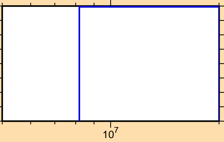
\sigma vs. E for ^{253}\text{No}(n,\text{pt})
