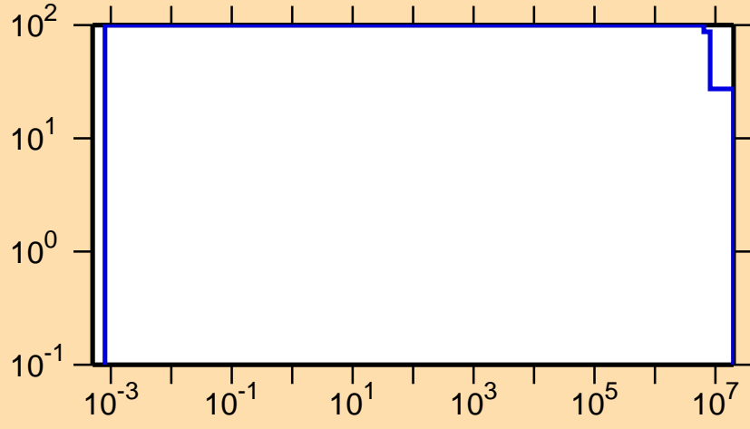
\Delta\sigma/\sigma vs. E for ^{253}\text{No}(n,p)
