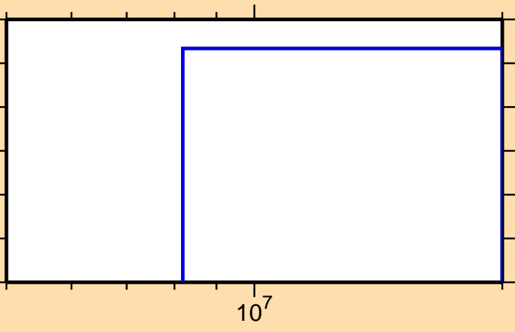
\sigma vs. E for ^{253}\text{No}(n,\text{He}3)
