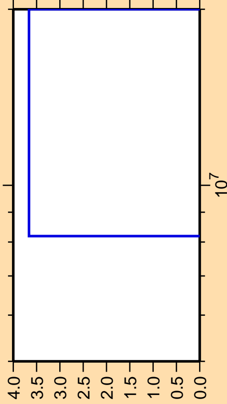
\Delta\sigma/\sigma vs. E for ^{253}\text{No}(\text{mt } 34)
