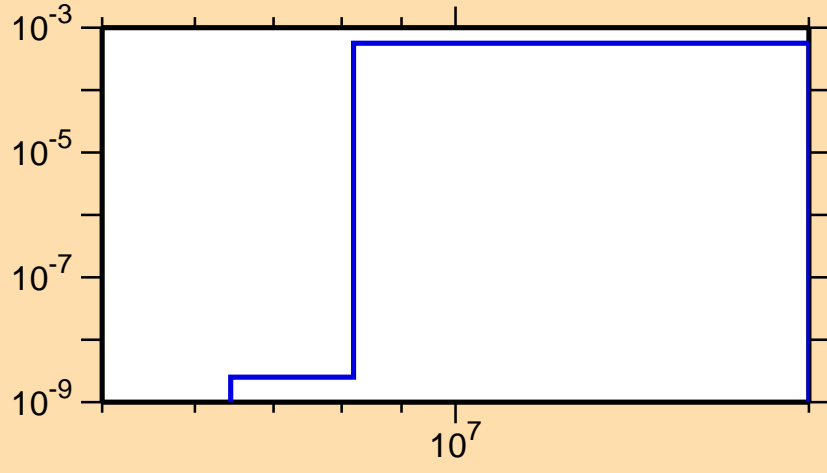
\sigma vs. E for ^{253}\text{No}(n,np)
