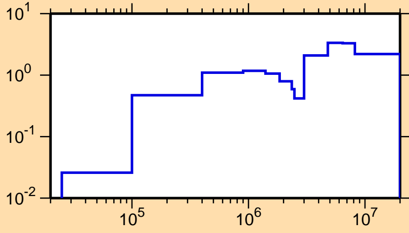
\sigma vs. E for ^{253}\text{No}(n,\text{inel.})
