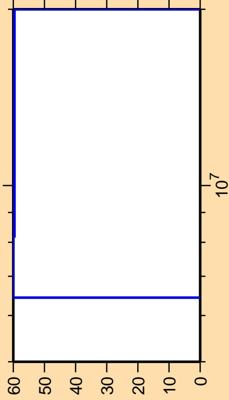
\Delta\sigma/\sigma vs. E for ^{253}\text{No}(n,n_1)
