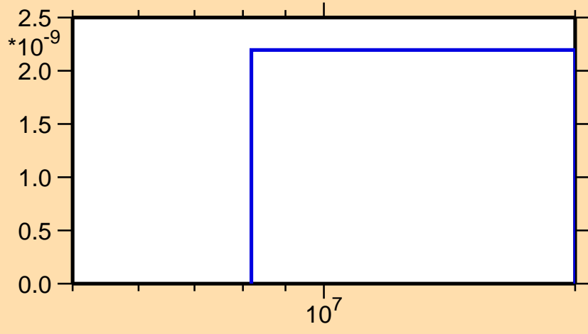
\sigma vs. E for ^{253}\text{No}(n,\text{nd})
