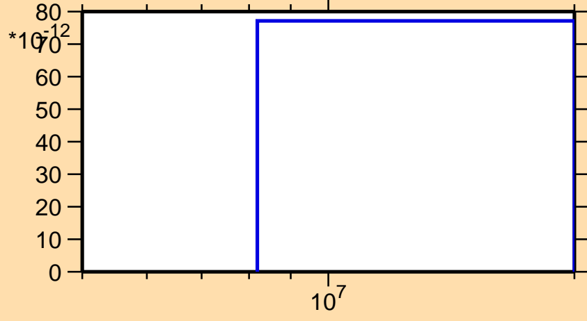
\sigma vs. E for ^{253}\text{No}(n,nt)
