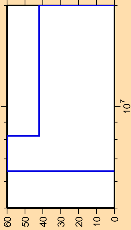
\Delta\sigma/\sigma vs. E for ^{253}\text{No}(n,np)
