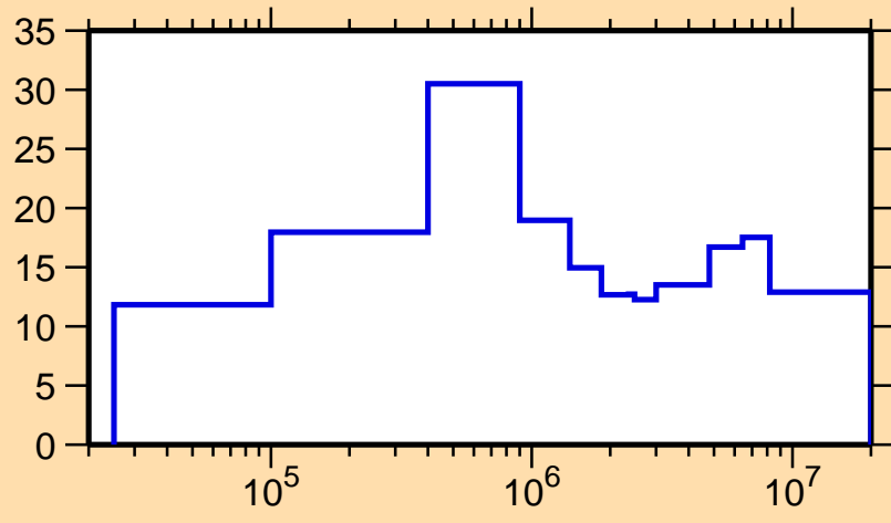
\Delta\sigma/\sigma vs. E for ^{253}\text{No}(n,\text{el.})
