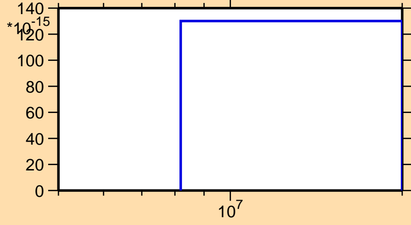
\sigma vs. E for ^{253}\text{No}(\text{mt117})
