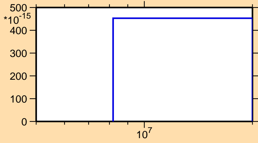
\sigma vs. E for ^{253}\text{No}(\text{mt } 45)
