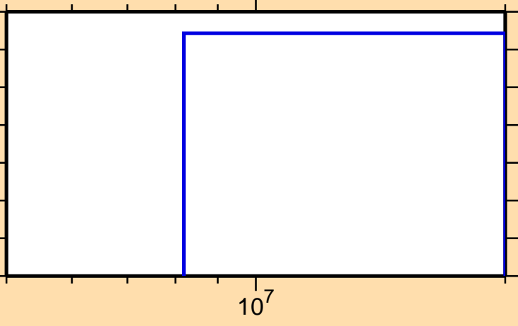
\sigma vs. E for ^{253}\text{No}(n,p\alpha)
