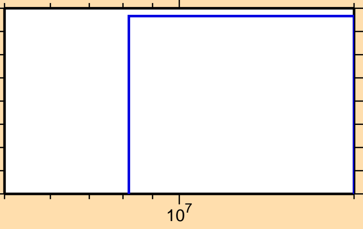
\sigma vs. E for ^{253}\text{No}(n,2np)
