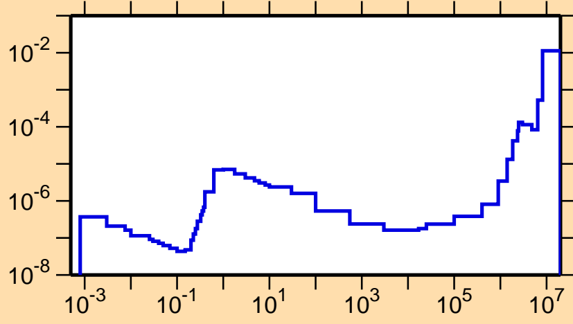
\sigma vs. E for ^{253}\text{No}(n,p)
