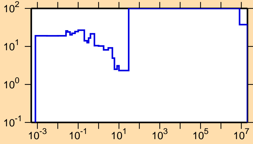
\Delta\sigma/\sigma vs. E for ^{253}\text{No}(n,f)
