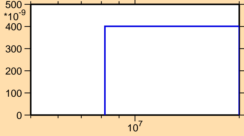
\sigma vs. E for ^{253}\text{No}(n,3n\alpha)
