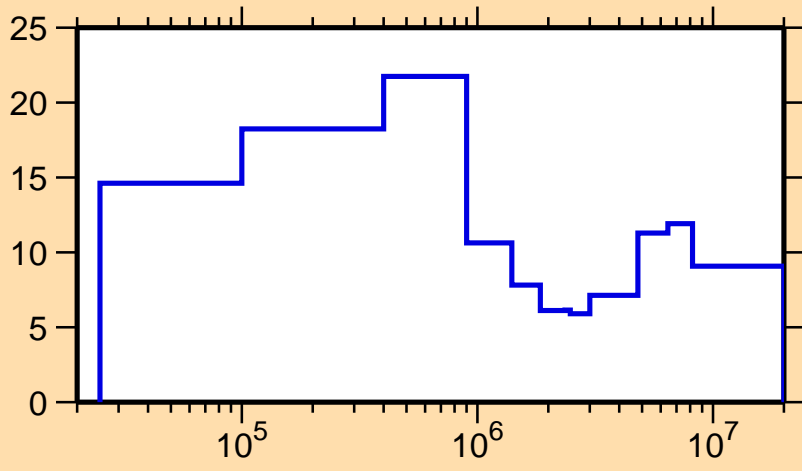
\Delta\sigma/\sigma vs. E for ^{253}\text{No}(n,\text{tot.})
