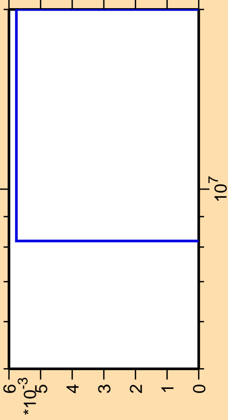
\Delta\sigma/\sigma vs. E for ^{253}\text{No}(n,\text{pt})
