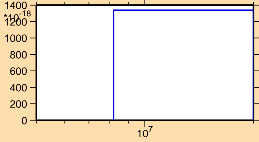
\sigma vs. E for ^{253}\text{No}(n,\text{pd})
