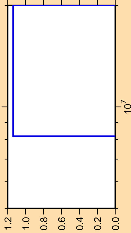
\Delta\sigma/\sigma vs. E for ^{253}\text{No}(\text{mt } 45)
