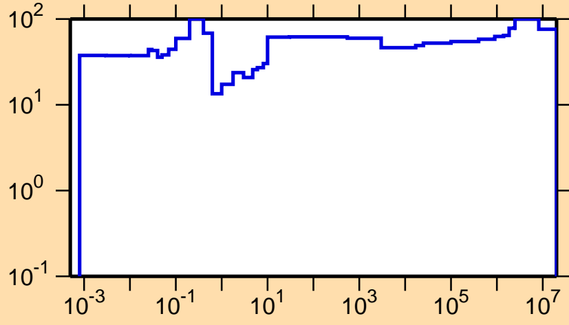
\Delta\sigma/\sigma vs. E for ^{253}\text{No}(n,\gamma)
