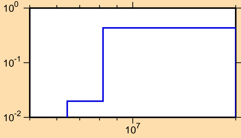
\sigma vs. E for ^{253}\text{No}(n,2n)
