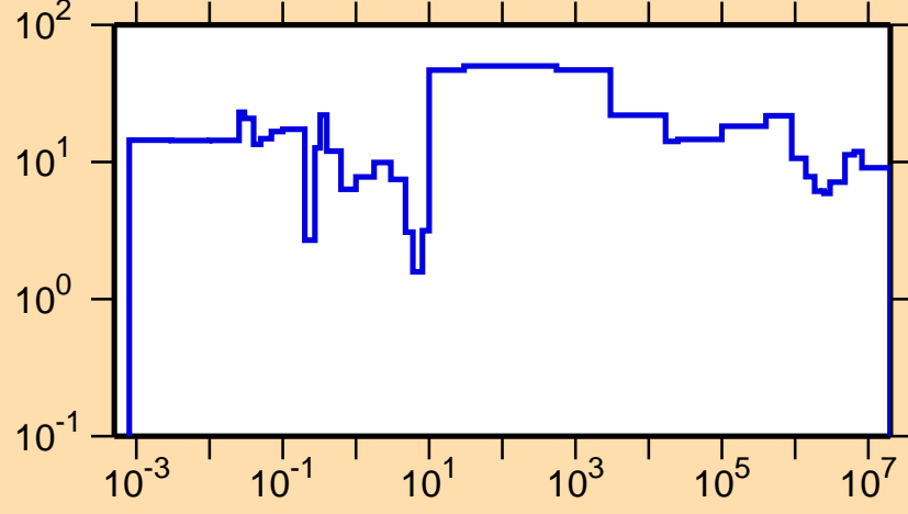
\Delta\sigma/\sigma vs. E for ^{253}\text{No}(n,\text{tot.})
