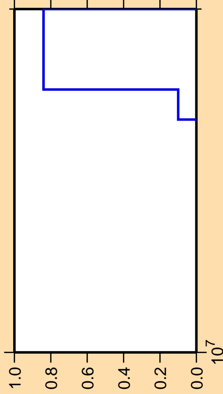
\Delta\sigma/\sigma vs. E for ^{254}\text{No}(\text{mt } 45)
