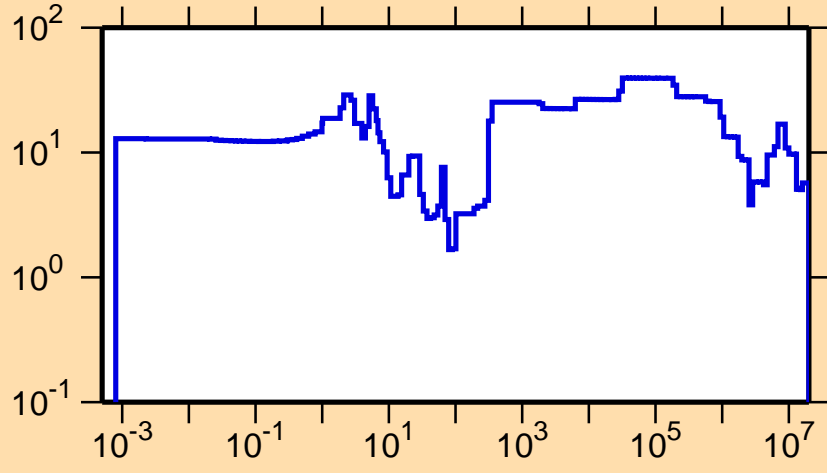
\Delta\sigma/\sigma vs. E for ^{254}\text{No}(n,tot.)
