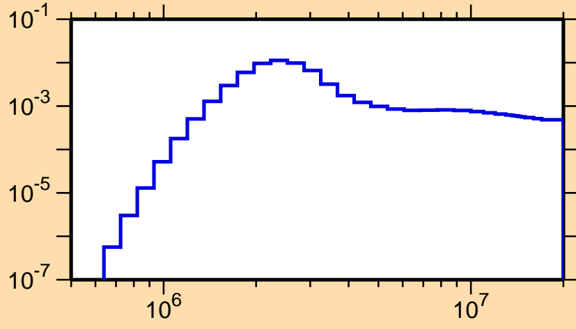
\sigma vs. E for ^{254}\text{No}(n,n_4)
