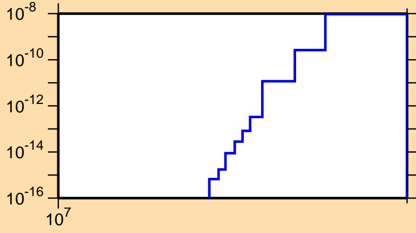
\sigma vs. E for ^{254}\text{No}(n,nt)
