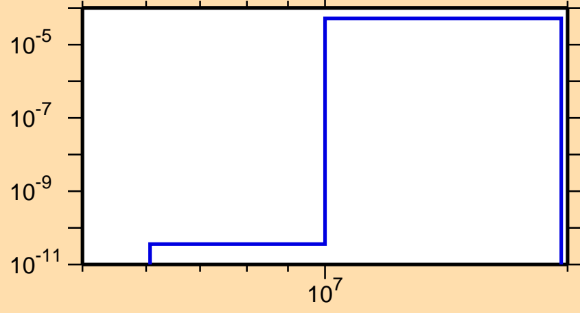
\sigma vs. E for ^{254}\text{No}(n,t)
