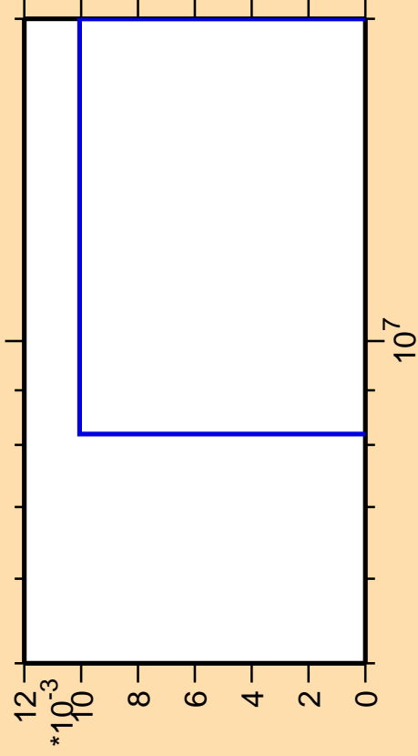
\Delta\sigma/\sigma vs. E for ^{254}\text{No}(n,3n\alpha)
