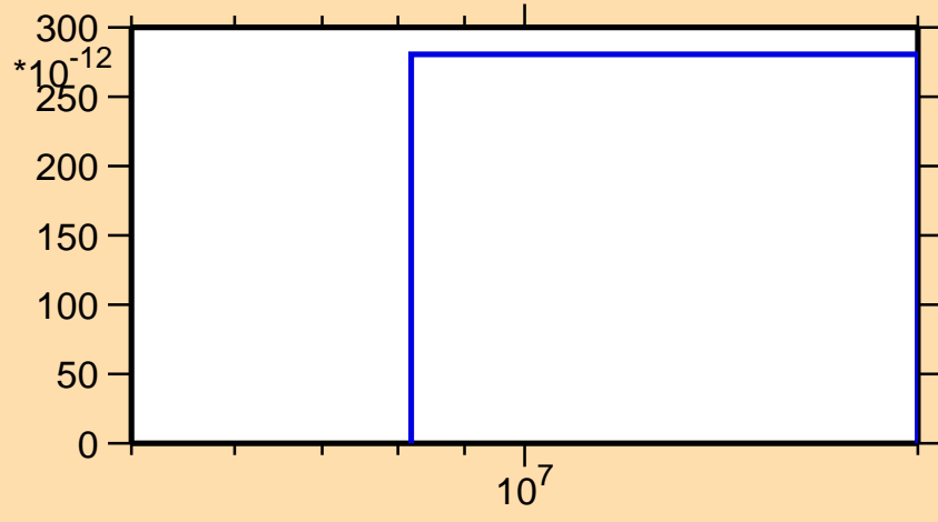
\sigma vs. E for ^{254}\text{No}(n,\text{nd})
