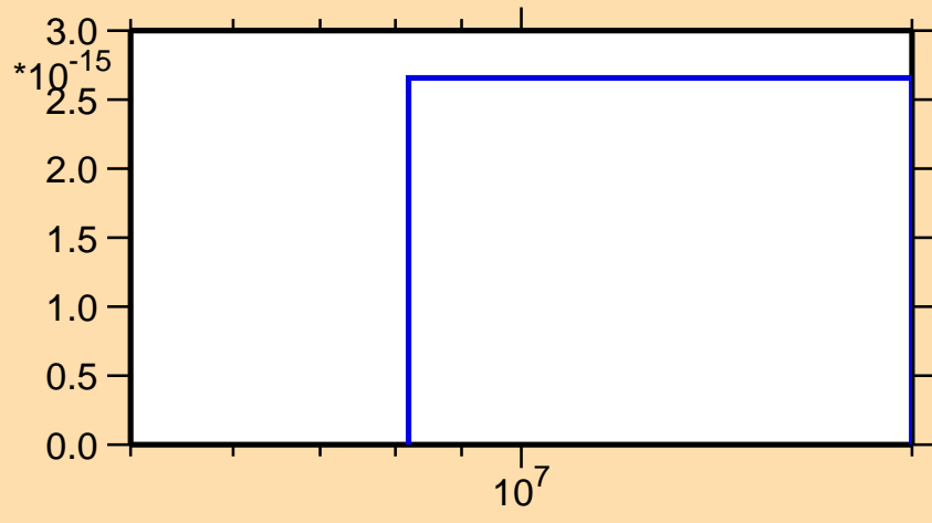
\sigma vs. E for ^{254}\text{No}(n,3n\alpha)
