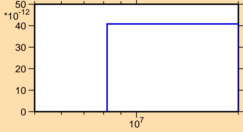
\sigma vs. E for ^{254}\text{No}(n,p\alpha)
