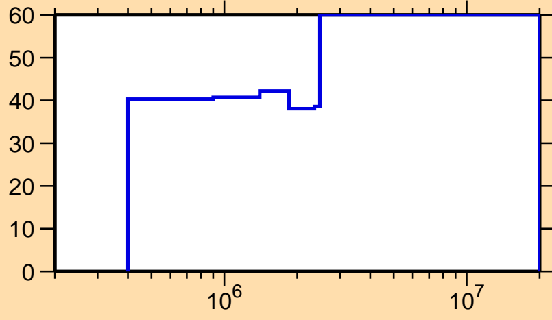
\Delta\sigma/\sigma vs. E for ^{254}\text{No}(n,n_1)
