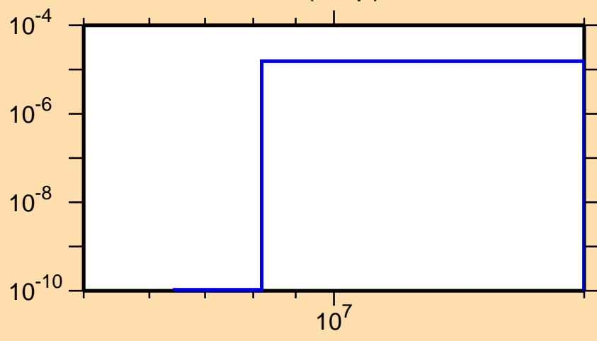
\sigma vs. E for ^{254}\text{No}(n,np)
