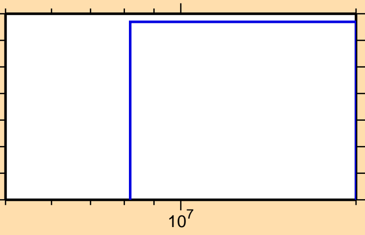
\sigma vs. E for ^{254}\text{No}(n,\text{He3})
