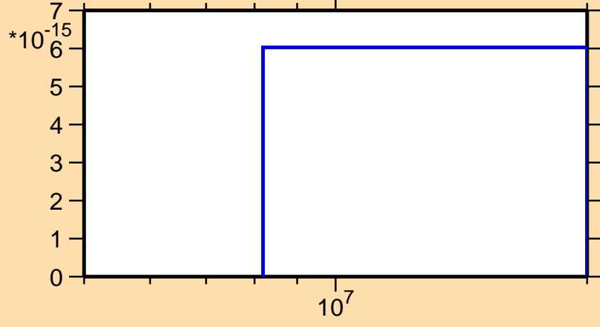
\sigma vs. E for ^{254}\text{No}(\text{mt117})
