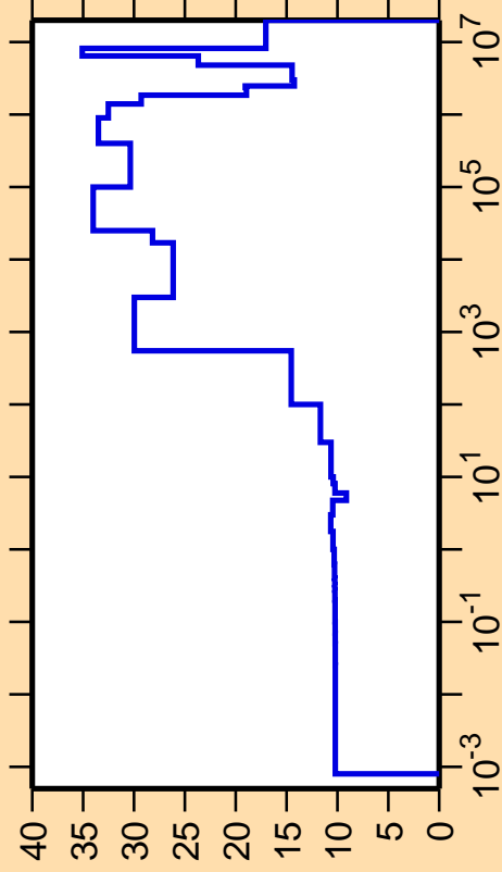
\Delta\sigma/\sigma vs. E for ^{254}\text{No}(n,\text{el.})
