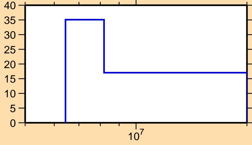
\Delta\sigma/\sigma vs. E for ^{254}\text{No}(n,\text{el.})
