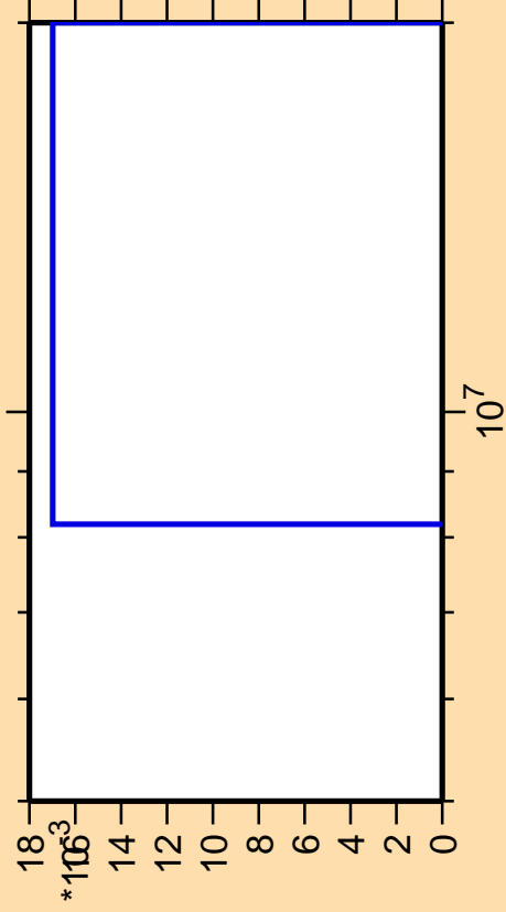
\Delta\sigma/\sigma vs. E for ^{254}\text{No}(\text{mt117})
