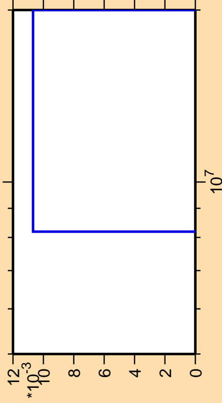
\Delta\sigma/\sigma vs. E for ^{254}\text{No}(\text{mt } 45)
