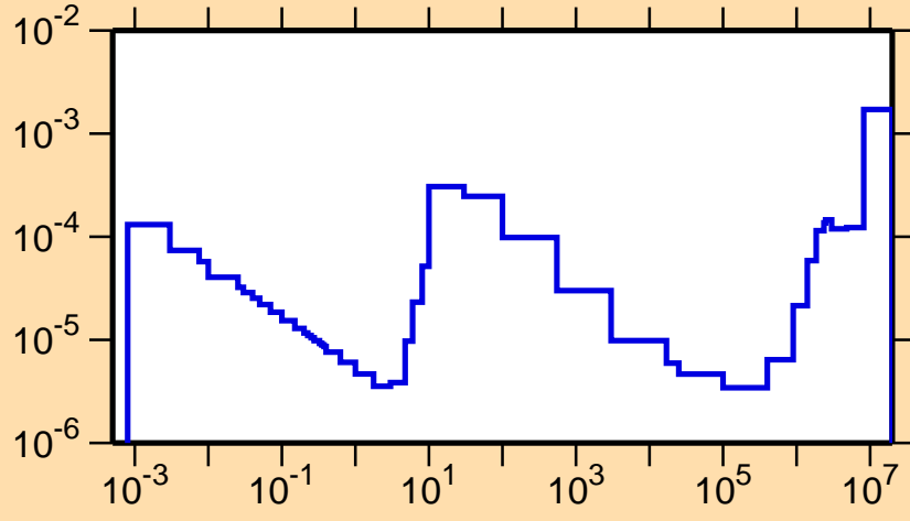
\sigma vs. E for ^{254}\text{No}(n,\alpha)
