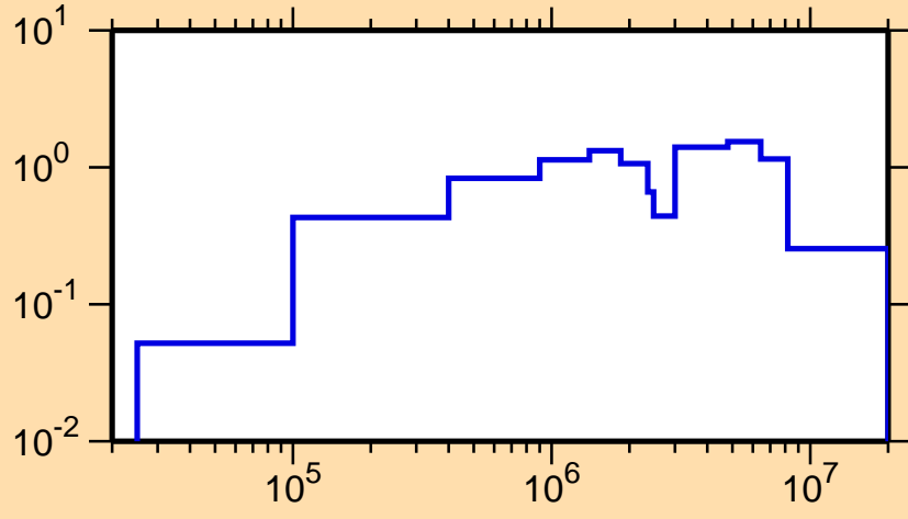
\sigma vs. E for ^{254}\text{No}(n,\text{inel.})
