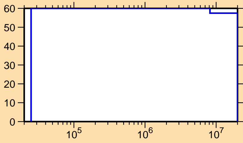
\Delta\sigma/\sigma vs. E for ^{254}\text{No}(n,f)
