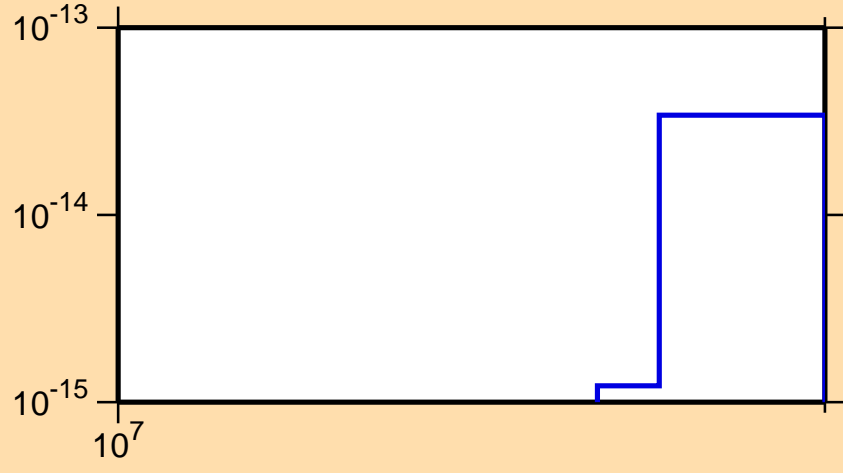
\sigma vs. E for ^{255}\text{No}(n,\text{pt})
