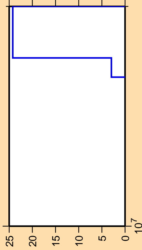
\Delta\sigma/\sigma vs. E for ^{255}\text{No} (mt 45)
