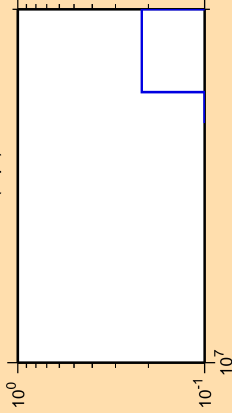
\Delta\sigma/\sigma vs. E for ^{255}\text{No}(n,\text{pt})
