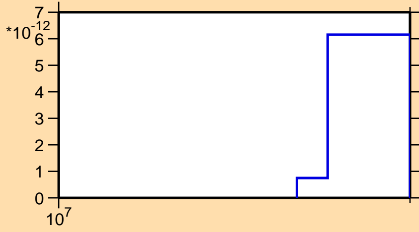
\sigma vs. E for ^{255}\text{No} (mt 45)
