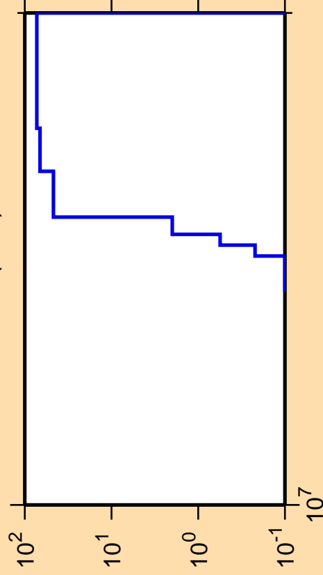
\Delta\sigma/\sigma vs. E for ^{259}\text{No}(n,\text{nt})
