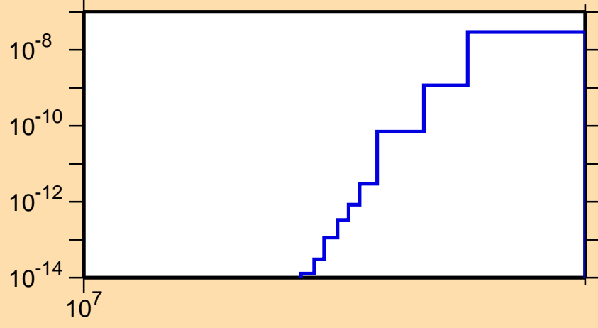
\sigma vs. E for ^{259}\text{No}(n,\text{nt})
