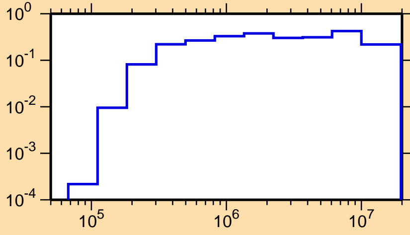
\sigma vs. E for ^{259}\text{No}(n,\text{inel.})
