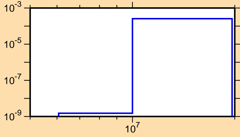
\sigma vs. E for ^{259}\text{No}(n,d)
