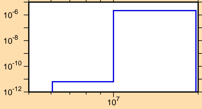
\sigma vs. E for ^{259}\text{No}(n,2n\alpha)
