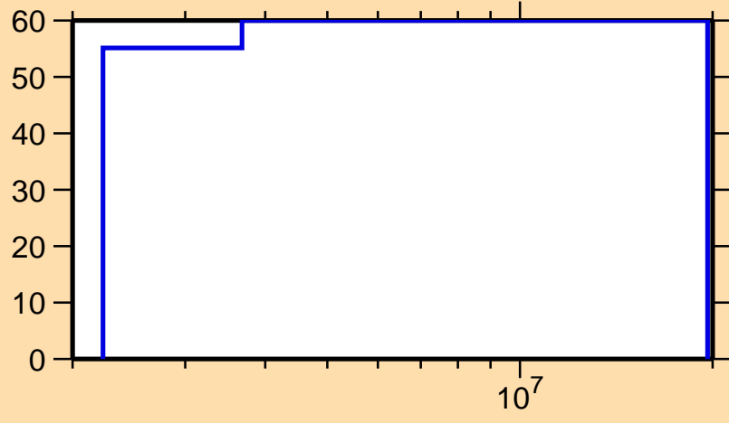
\Delta\sigma/\sigma vs. E for ^{259}\text{No}(n,p)
