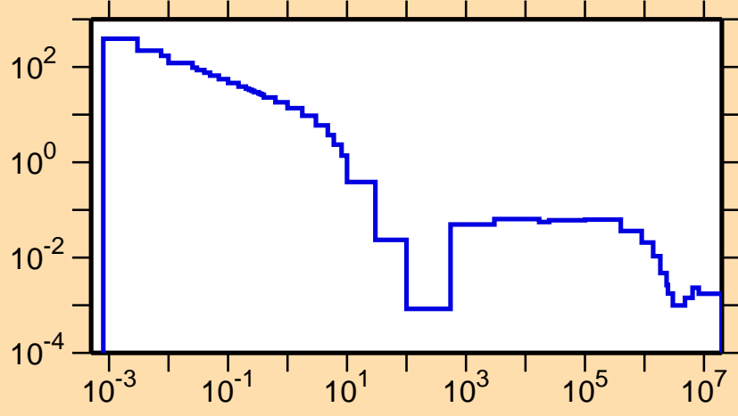
\sigma vs. E for ^{259}\text{No}(n,\gamma)
