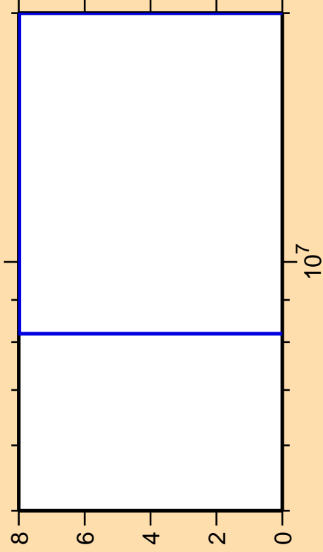
\Delta\sigma/\sigma vs. E for ^{259}\text{No}(n,2np)
