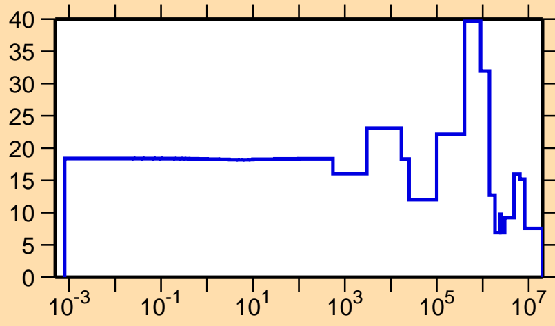
\Delta\sigma/\sigma vs. E for ^{259}\text{No}(n,el.)
