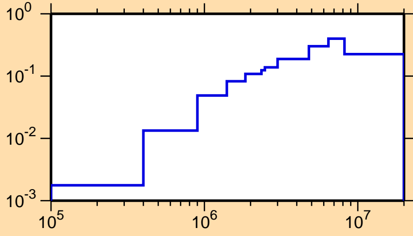
\sigma vs. E for ^{259}\text{No}(n,n\text{cont.})
