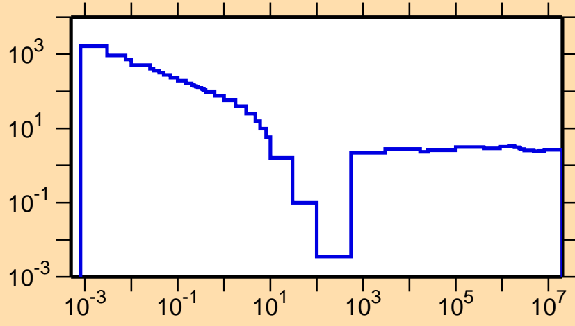
\sigma vs. E for ^{259}\text{No}(n,f)
