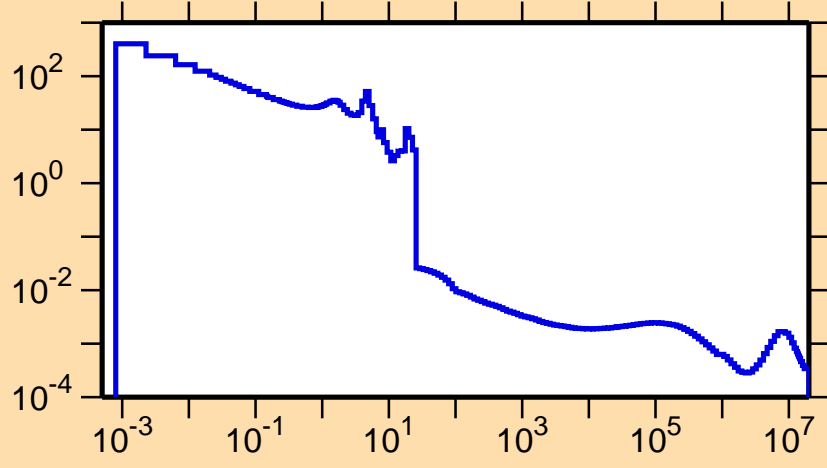
\sigma vs. E for ^{263}\text{No}(n,\gamma)
