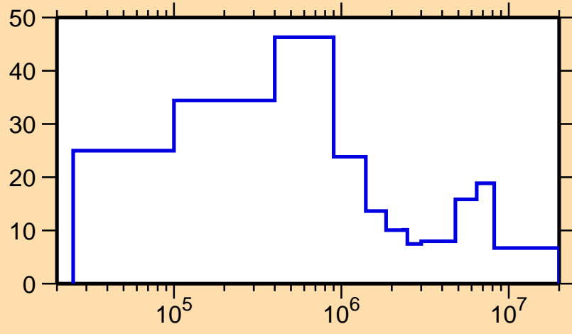
\Delta\sigma/\sigma vs. E for ^{263}\text{No}(n,\text{el.})
