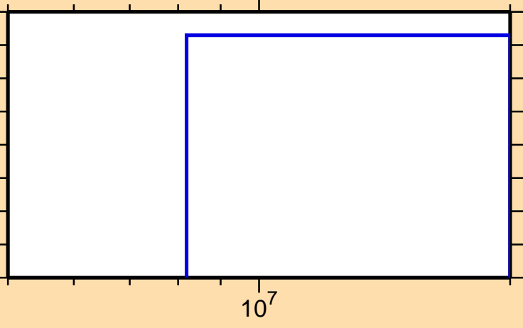
\sigma vs. E for ^{263}\text{No}(n,nt)
