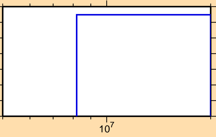
\sigma vs. E for ^{263}\text{No}(n,3n)
