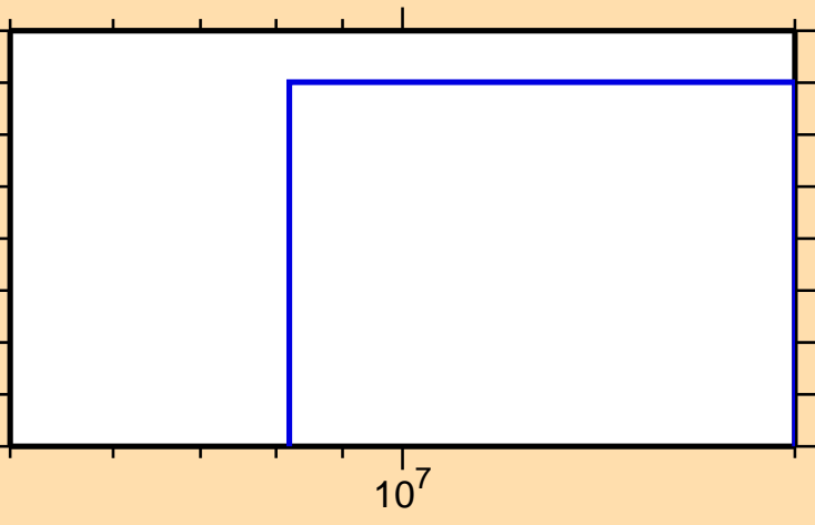
\sigma vs. E for ^{263}\text{No}(n,\text{nd})
