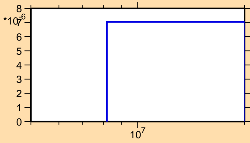
\sigma vs. E for ^{263}\text{No}(n,d)
