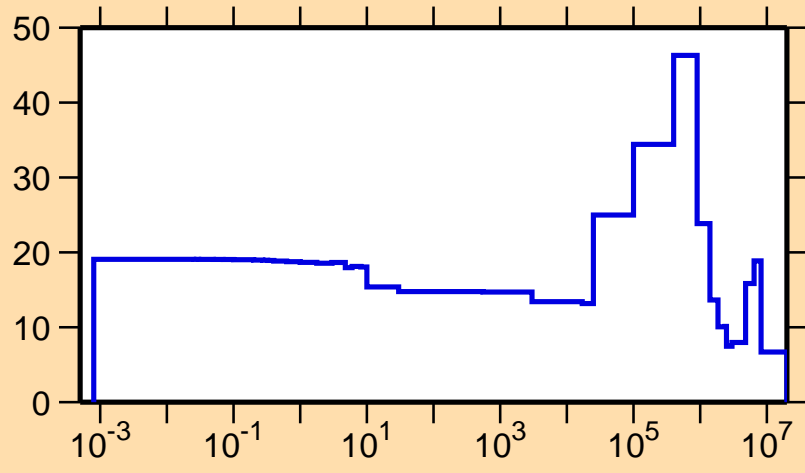
\Delta\sigma/\sigma vs. E for ^{263}\text{No}(n,el.)
