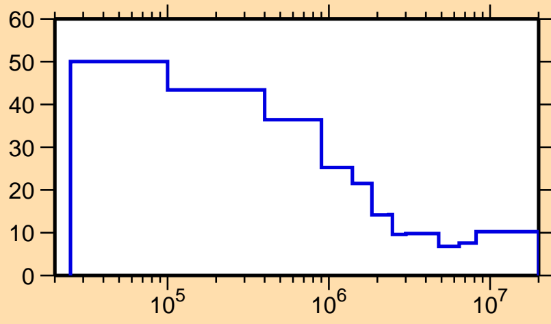
\Delta\sigma/\sigma vs. E for ^{263}\text{No}(n,f)
