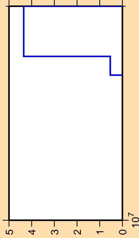
\Delta\sigma/\sigma vs. E for ^{264}\text{No}(n,\text{He}3)
