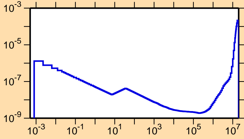
\sigma vs. E for ^{264}\text{No}(n,\alpha)
