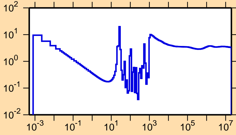
\sigma vs. E for ^{264}\text{No}(n,f)
