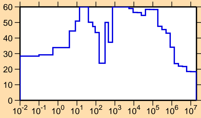
\Delta\sigma/\sigma vs. E for ^{264}\text{No}(n,f)
