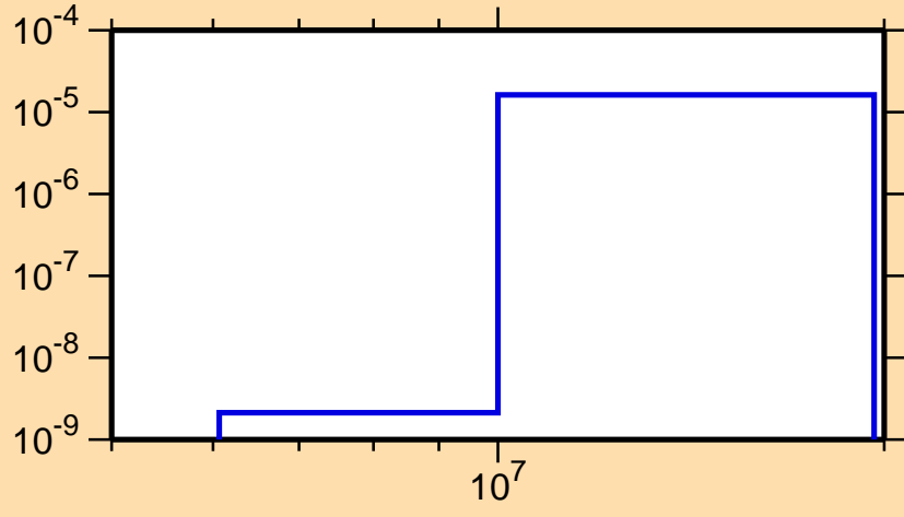
\sigma vs. E for ^{264}\text{No}(n,n\alpha)
