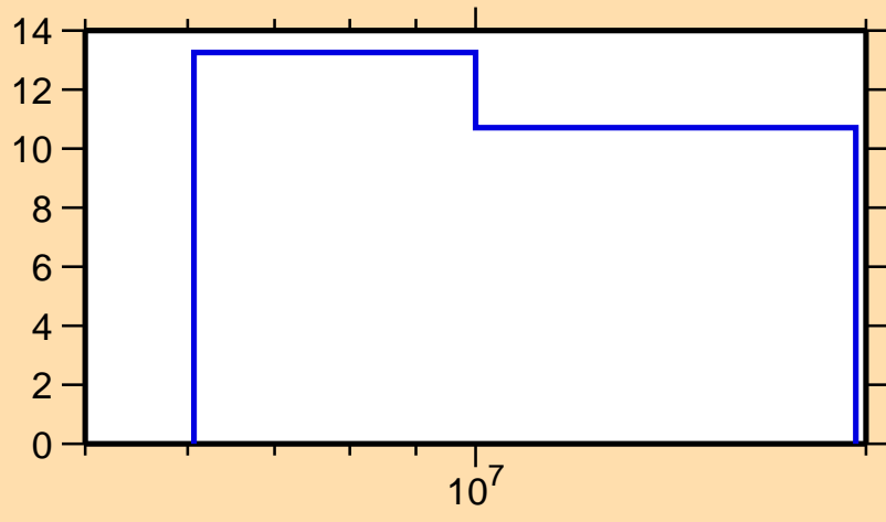
\Delta\sigma/\sigma vs. E for ^{264}\text{No}(n,\text{nonel.})
