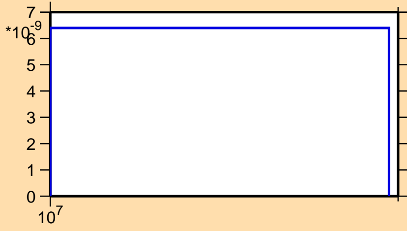
\sigma vs. E for ^{264}\text{No}(n,2n\alpha)
