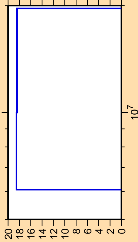
\Delta\sigma/\sigma vs. E for ^{264}\text{No}(n,f)
