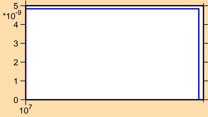
\sigma vs. E for ^{264}\text{No}(n,nt)
