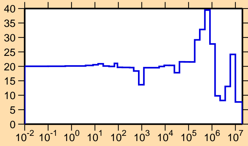
\Delta\sigma/\sigma vs. E for ^{264}\text{No}(n,\text{el.})
