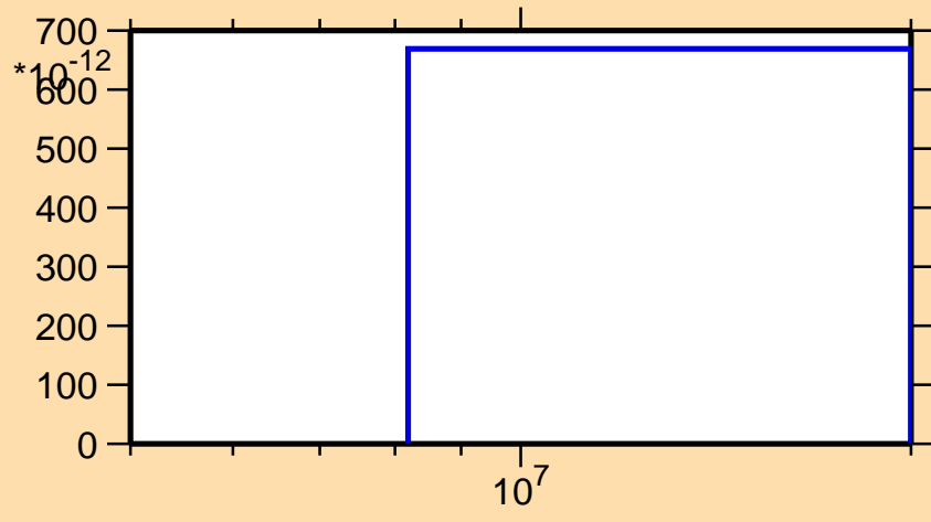
\sigma vs. E for ^{264}\text{No}(n,2np)
