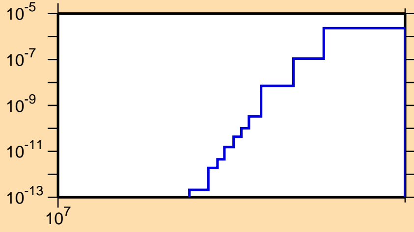
\sigma vs. E for ^{228}\text{Np}(n,nt)
