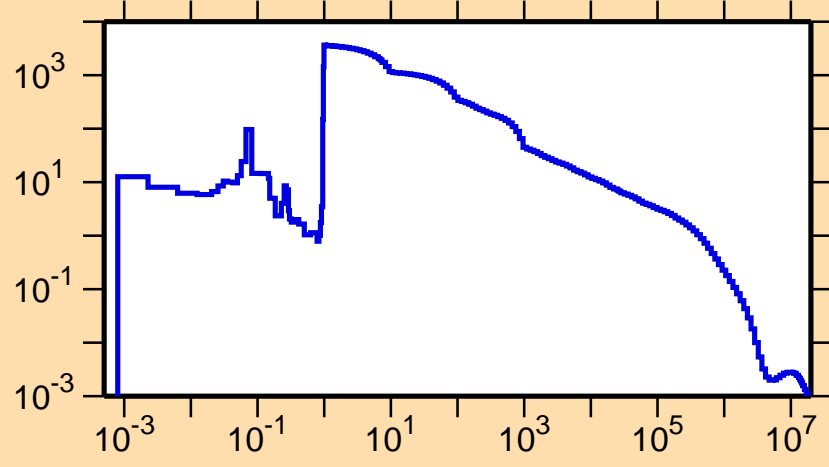
\sigma vs. E for ^{228}\text{Np}(n,\gamma)
