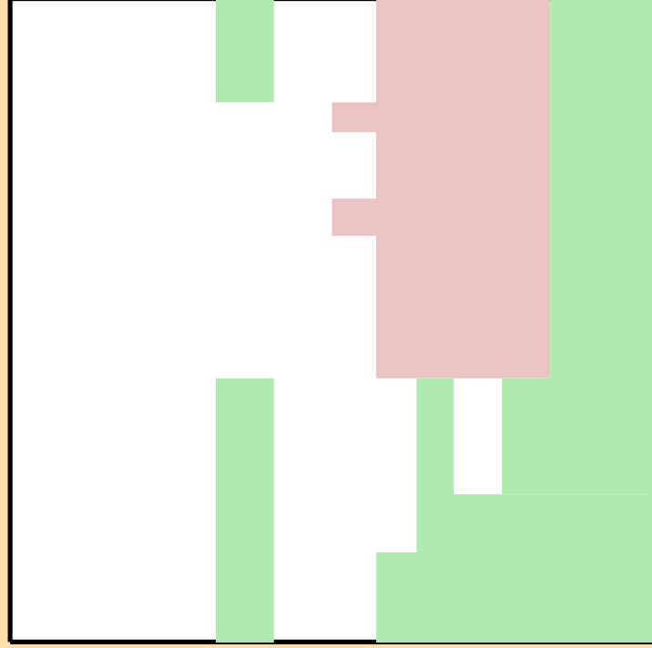
\Delta\sigma/\sigma vs. E for ^{228}\text{Np}(n,2n)
