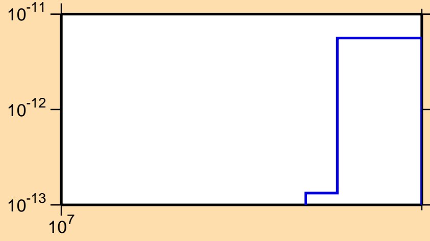
\sigma vs. E for ^{228}\text{Np} (mt 34)
