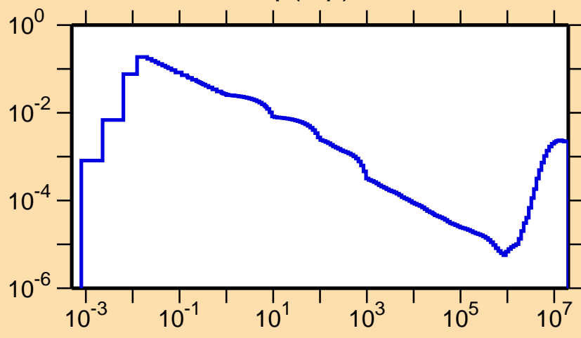
\sigma vs. E for ^{228}\text{Np}(n,p)
