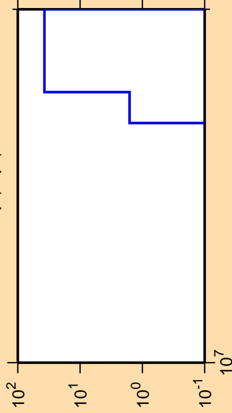
\Delta\sigma/\sigma vs. E for ^{228}\text{Np}(n,\text{pt})
