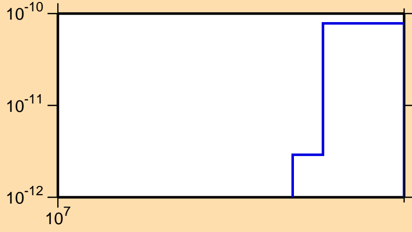
\sigma vs. E for ^{228}\text{Np}(n,\text{pd})
