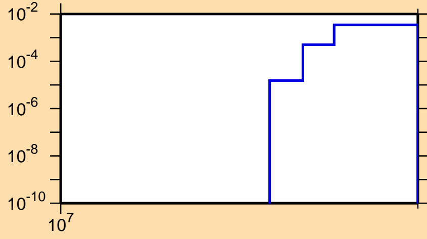
\sigma vs. E for ^{228}\text{Np}(n,3n\alpha)
