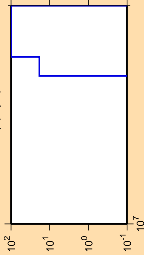
\Delta\sigma/\sigma vs. E for ^{228}\text{Np}(n,\text{pd})
