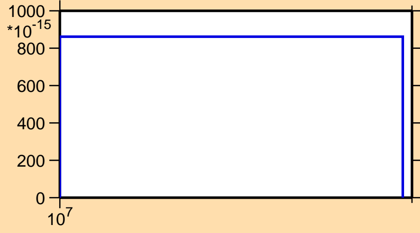
\sigma vs. E for ^{228}\text{Np}(n,\text{pd})
