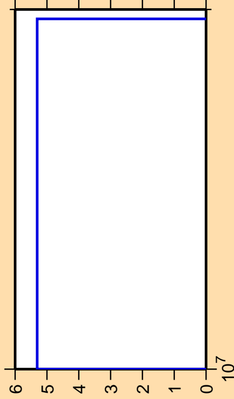
\Delta\sigma/\sigma vs. E for ^{228}\text{Np}(n,\text{pd})
