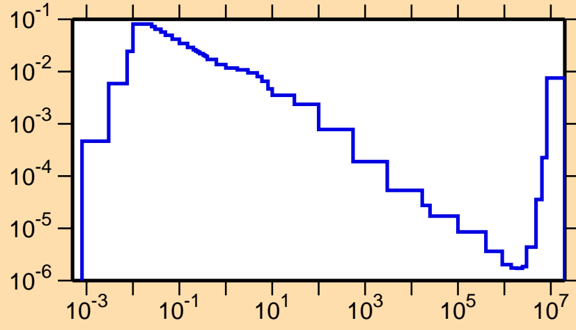
\sigma vs. E for ^{228}\text{Np}(n,\alpha)
