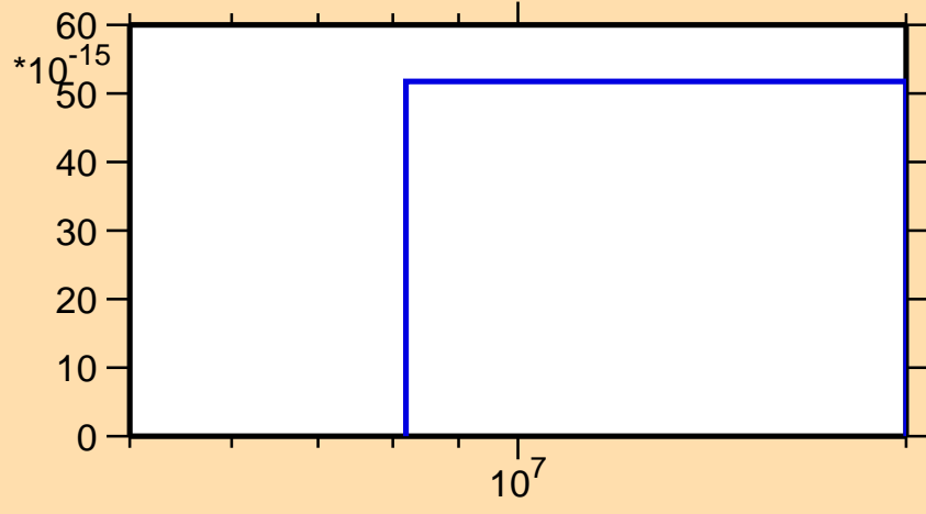
\sigma vs. E for ^{228}\text{Np}(\text{mt } 34)
