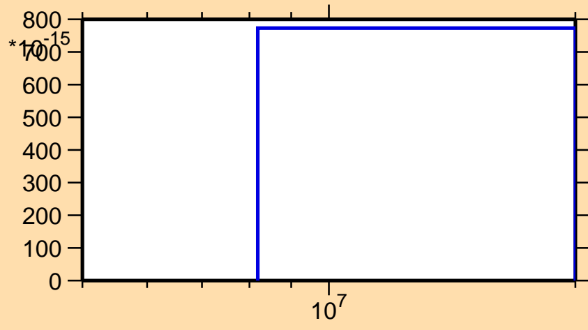
\sigma vs. E for ^{228}\text{Np}(n,pd)
