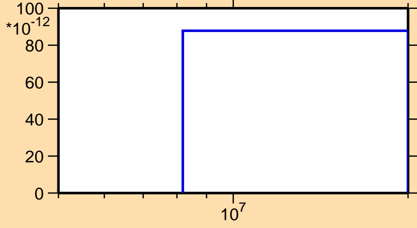
\sigma vs. E for ^{228}\text{Np}(\text{mt117})
