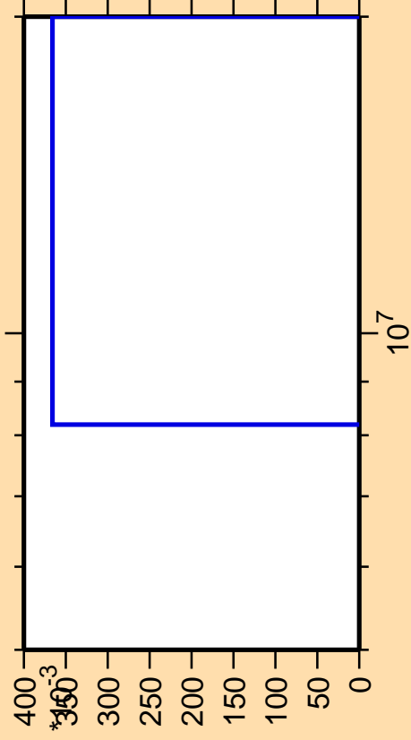
\Delta\sigma/\sigma vs. E for ^{228}\text{Np}(n,\text{pt})
