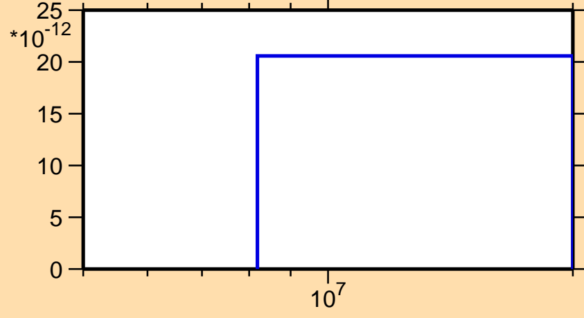
\sigma vs. E for ^{228}\text{Np}(\text{mt } 45)
