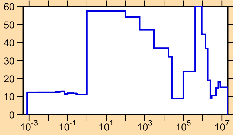
\Delta\sigma/\sigma vs. E for ^{228}\text{Np}(n,\text{el.})
