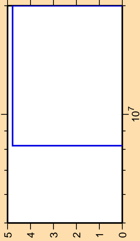
\Delta\sigma/\sigma vs. E for ^{228}\text{Np}(n,pd)
