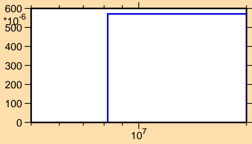
\sigma vs. E for ^{228}\text{Np}(n,3n)
