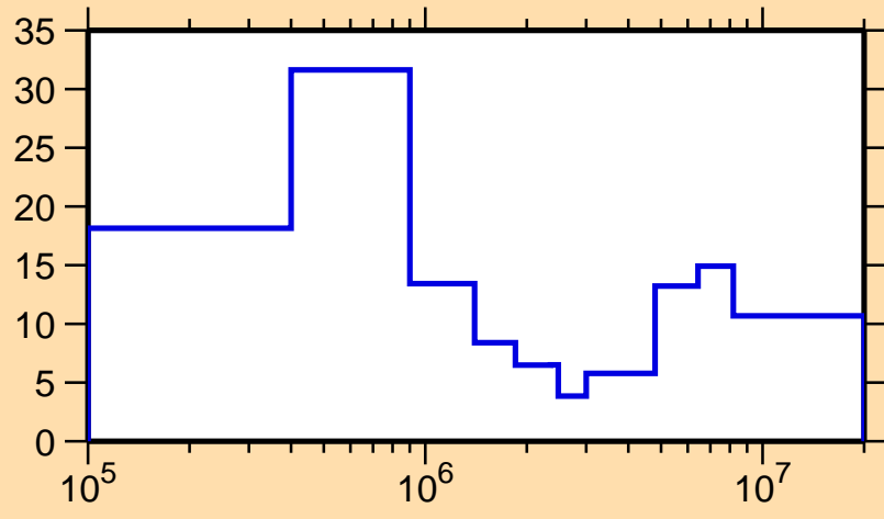
\Delta\sigma/\sigma vs. E for ^{228}\text{Np}(n,\text{tot.})
