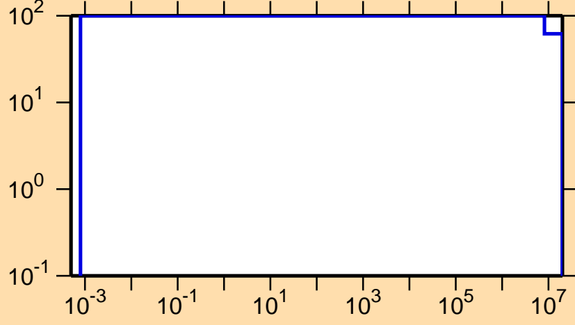
\Delta\sigma/\sigma vs. E for ^{228}\text{Np}(n,p)
