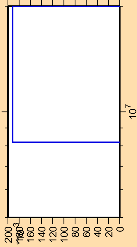
\Delta\sigma/\sigma vs. E for ^{228}\text{Np}(\text{mt } 34)
