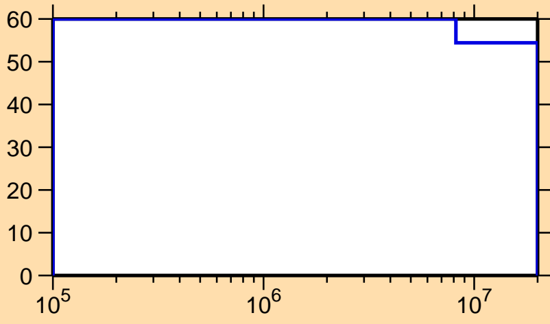
\Delta\sigma/\sigma vs. E for ^{228}\text{Np}(n,f)
