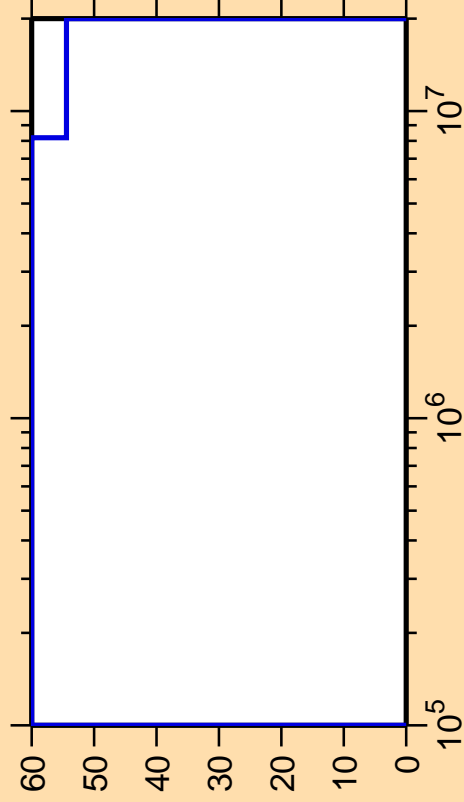
\Delta\sigma/\sigma vs. E for ^{228}\text{Np}(n,f)
