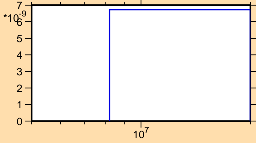
\sigma vs. E for ^{228}\text{Np}(n,\text{He3})
