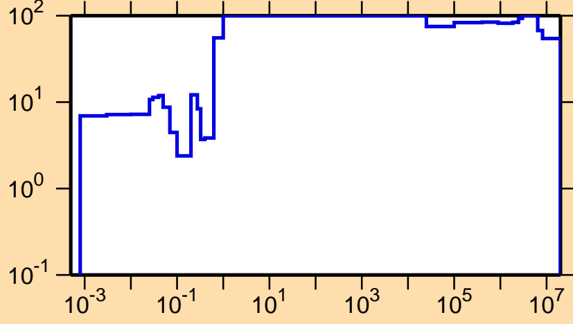
\Delta\sigma/\sigma vs. E for ^{228}\text{Np}(n,f)
