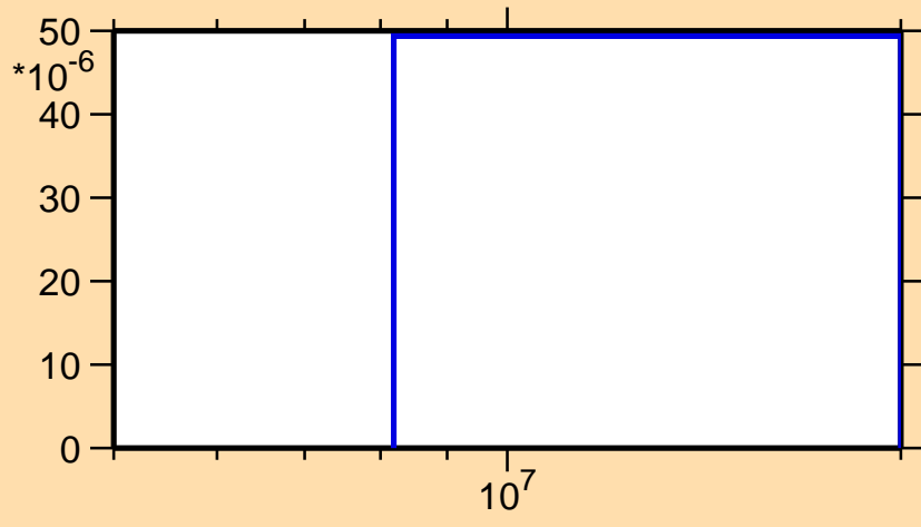
\sigma vs. E for ^{228}\text{Np}(n,3n\alpha)
