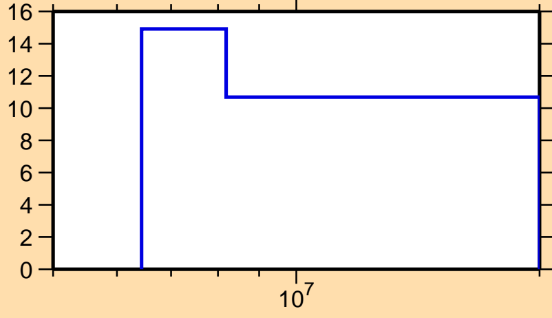
\Delta\sigma/\sigma vs. E for ^{228}\text{Np}(n,\text{tot.})
