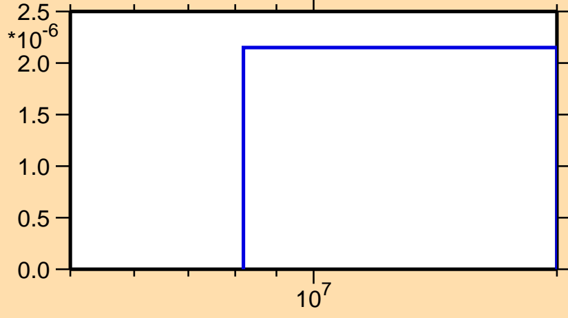
\sigma vs. E for ^{228}\text{Np}(n,2np)
