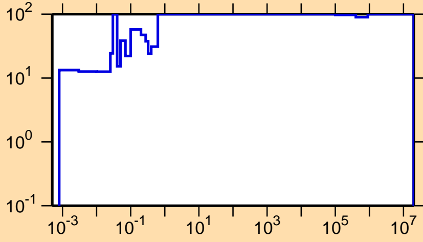
\Delta\sigma/\sigma vs. E for ^{228}\text{Np}(n,\gamma)
