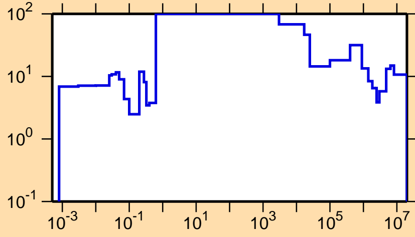
\Delta\sigma/\sigma vs. E for ^{228}\text{Np}(n,tot.)
