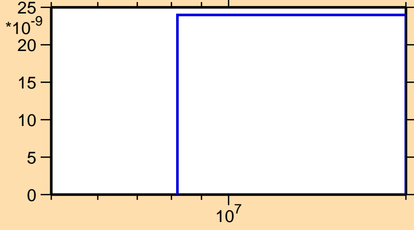
\sigma vs. E for ^{228}\text{Np}(n,nt)
