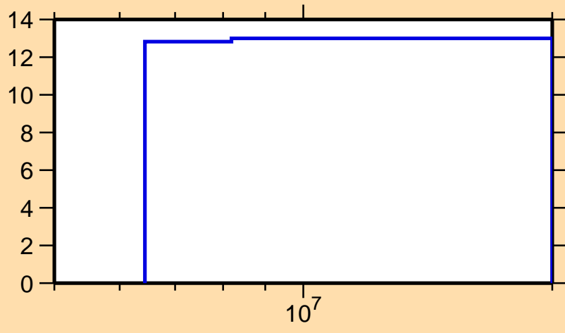
\Delta\sigma/\sigma vs. E for ^{228}\text{Np}(n,\text{nonel.})
