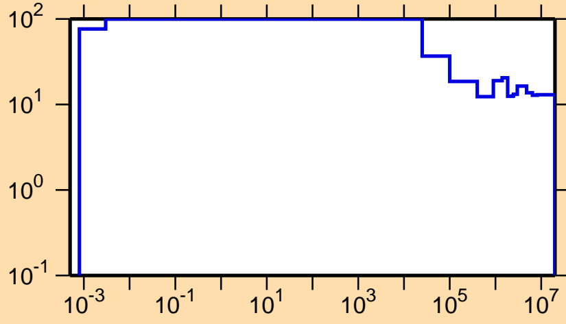
\Delta\sigma/\sigma vs. E for ^{228}\text{Np}(n,\text{nonel.})
