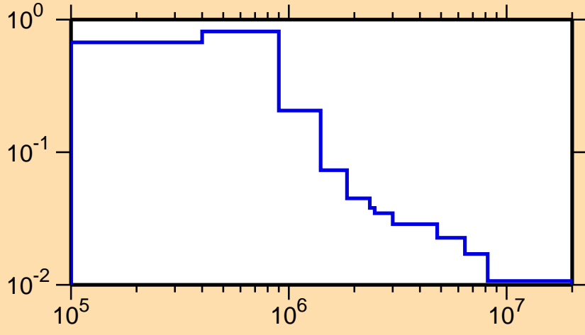
\sigma vs. E for ^{228}\text{Np}(n,\text{inel.})
