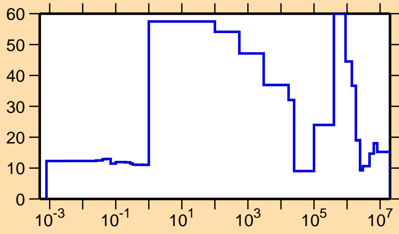
\Delta\sigma/\sigma vs. E for ^{228}\text{Np}(n,\text{el.})
