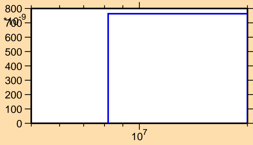
\sigma vs. E for ^{228}\text{Np}(n,nd)
