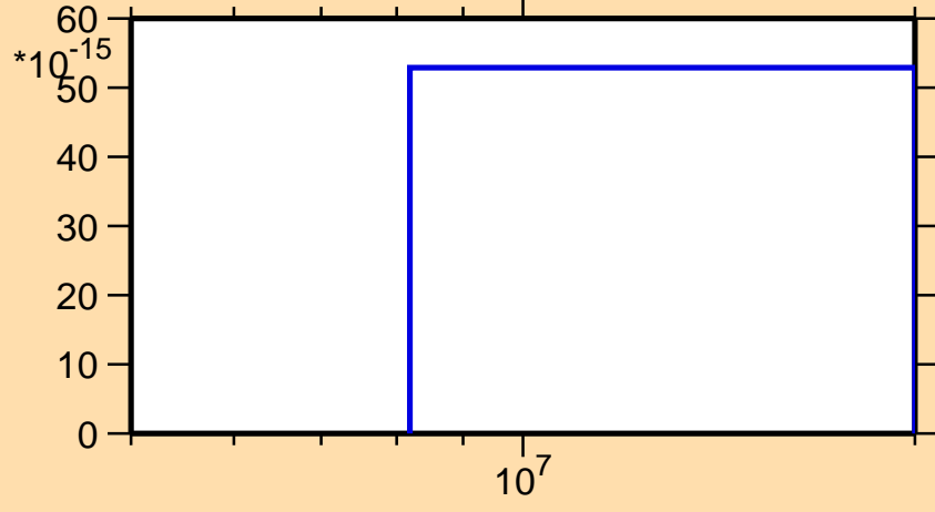
\sigma vs. E for ^{228}\text{Np}(n,\text{pt})
