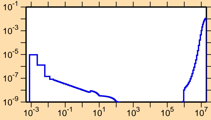
\sigma vs. E for ^{229}\text{Np}(n,\alpha)
