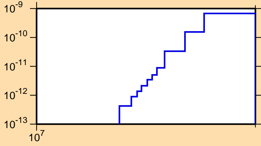
\sigma vs. E for ^{229}\text{Np}(\text{mt117})
