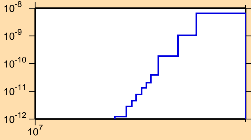
\sigma vs. E for ^{229}\text{Np} (mt 45)
