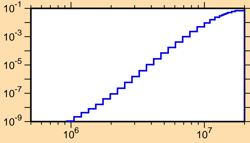
\sigma vs. E for ^{229}\text{Np}(n,p)
