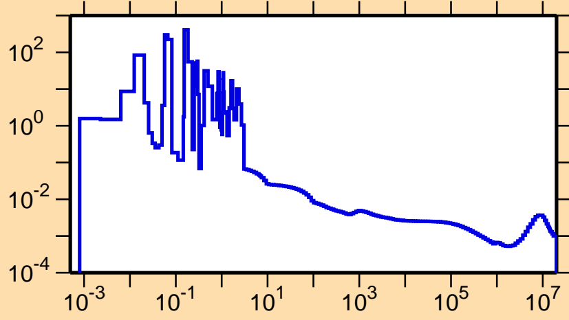
\sigma vs. E for ^{229}\text{Np}(n,\gamma)
