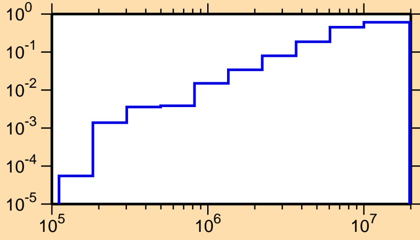
\sigma vs. E for ^{229}\text{Np}(n,\text{inel.})
