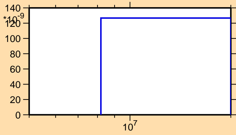
\sigma vs. E for ^{229}\text{Np}(n,2n\alpha)
