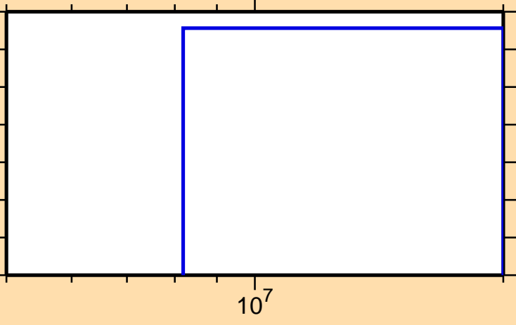
\sigma vs. E for ^{229}\text{Np}(n,\text{nd})
