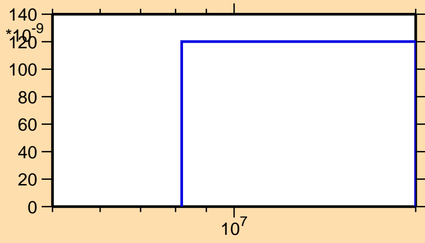
\sigma vs. E for ^{229}\text{Np}(n,2np)
