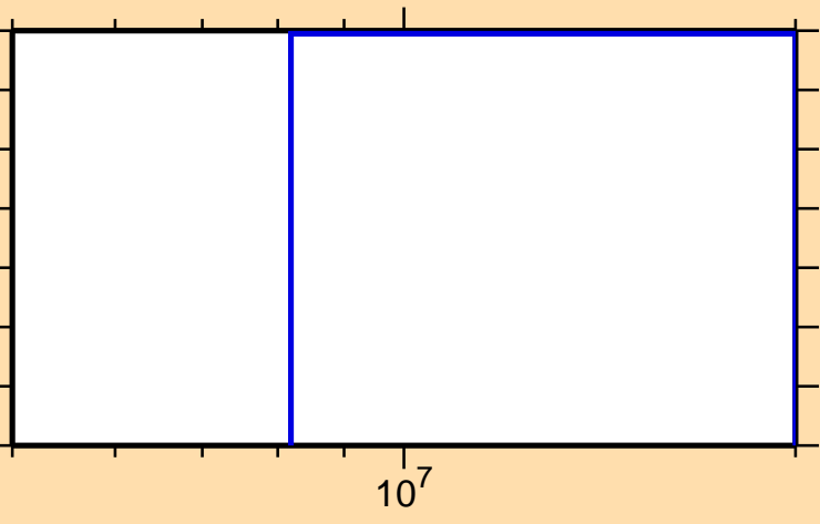
\sigma vs. E for ^{229}\text{Np}(n,\text{He}3)
