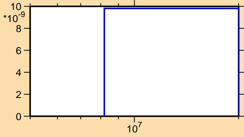
\sigma vs. E for ^{230}\text{Np}(n,nt)
