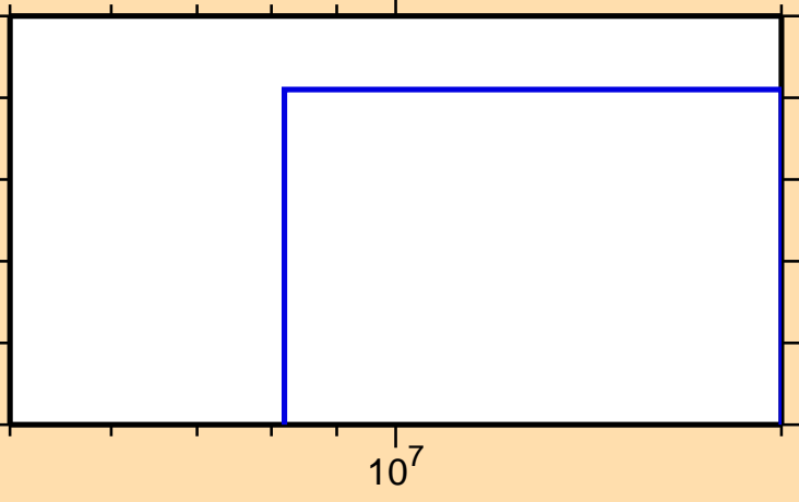
\sigma vs. E for ^{230}\text{Np}(n,nd)
