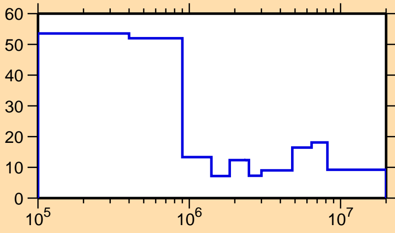
\Delta\sigma/\sigma vs. E for ^{230}\text{Np}(n,\text{tot.})
