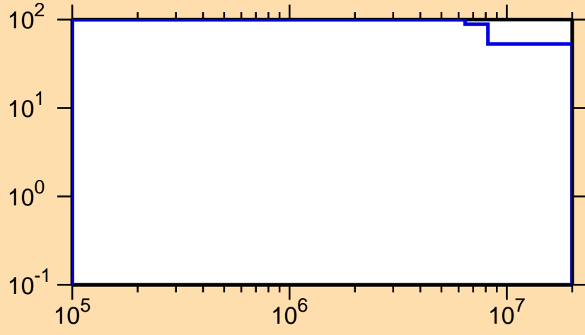
\Delta\sigma/\sigma vs. E for ^{230}\text{Np}(n,n\text{cont.})
