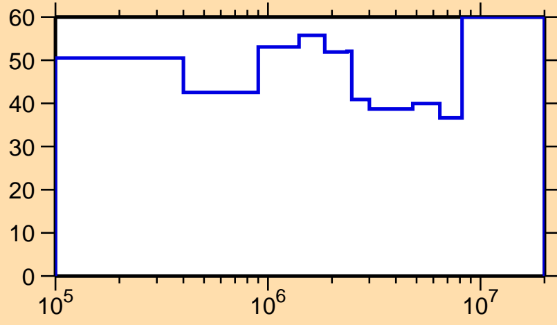
\Delta\sigma/\sigma vs. E for ^{230}\text{Np}(n,f)
