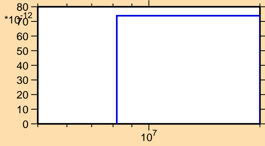
\sigma vs. E for ^{230}\text{Np}(\text{mt117})
