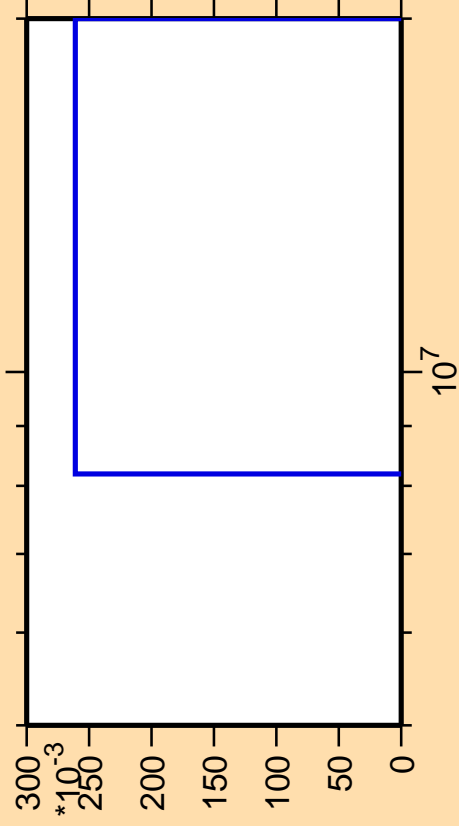
\Delta\sigma/\sigma vs. E for ^{230}\text{Np}(n,3n\alpha)
