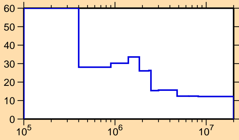
\Delta\sigma/\sigma vs. E for ^{230}\text{Np}(n,\text{nonel.})
