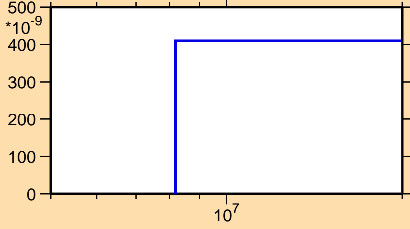
\sigma vs. E for ^{230}\text{Np}(n,nd)
