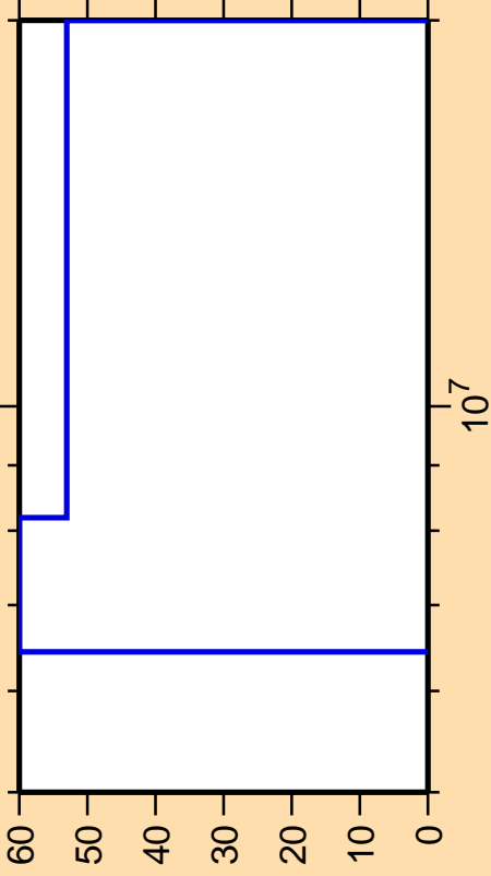
\Delta\sigma/\sigma vs. E for ^{230}\text{Np}(n,n\text{cont.})
