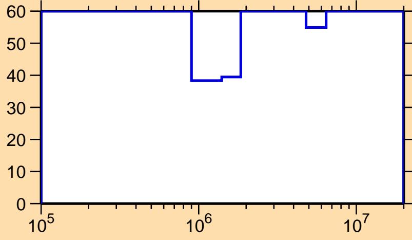
\Delta\sigma/\sigma vs. E for ^{230}\text{Np}(n,n_1)
