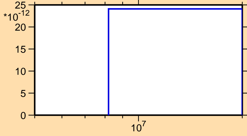
\sigma vs. E for ^{230}\text{Np}(n,p\alpha)
