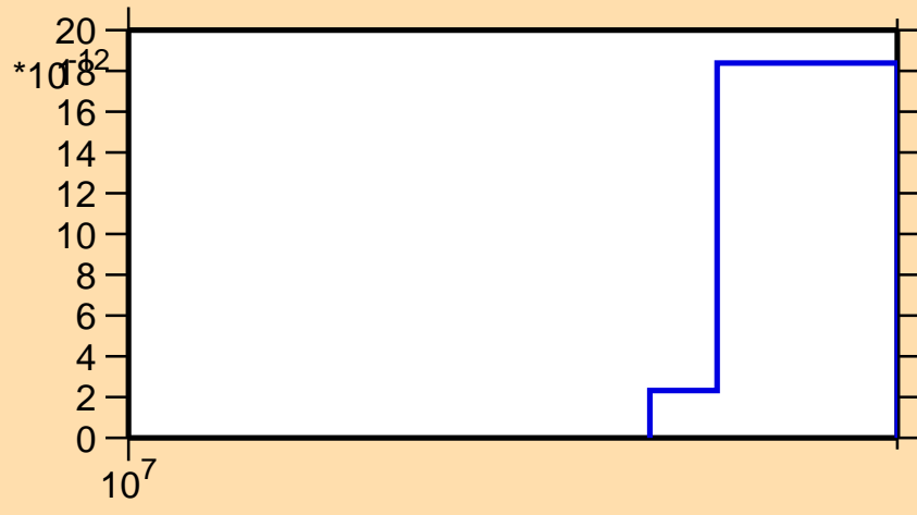
\sigma vs. E for ^{231}\text{Np}(\text{mt } 45)
