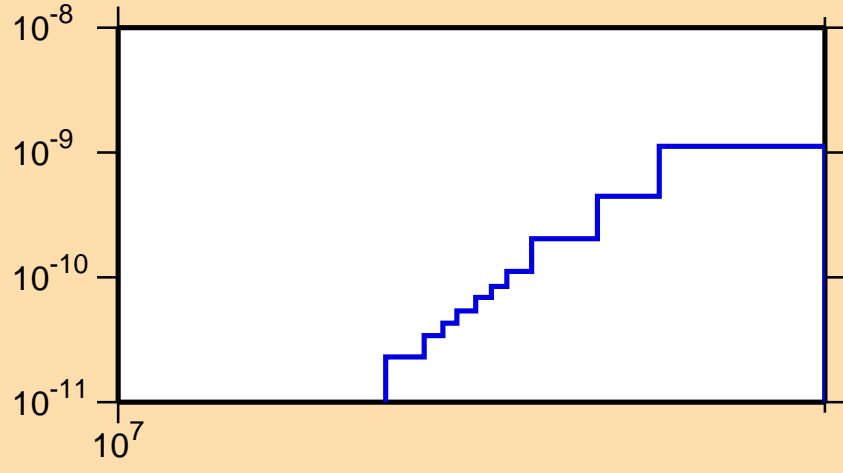
\sigma vs. E for ^{231}\text{Np}(n,p\alpha)
