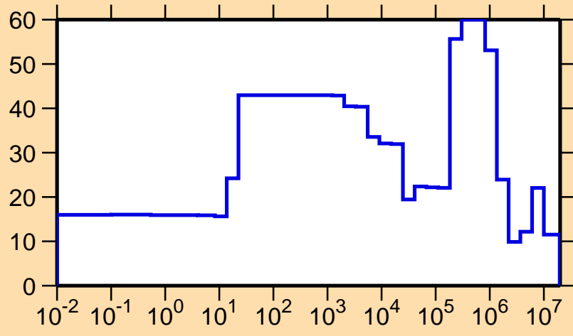
\Delta\sigma/\sigma vs. E for ^{231}\text{Np}(n,\text{el.})
