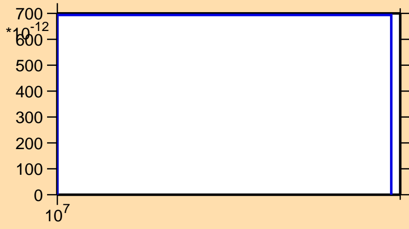
\sigma vs. E for ^{231}\text{Np}(n,\text{He}3)
