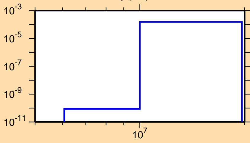
\sigma vs. E for ^{231}\text{Np}(n,t)
