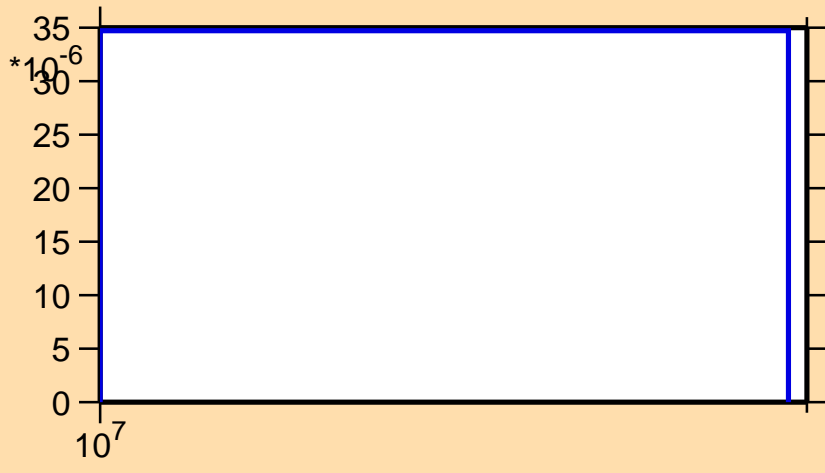
\sigma vs. E for ^{231}\text{Np}(n,3n)
