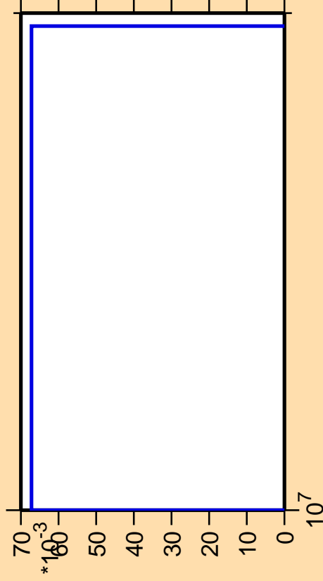
\Delta\sigma/\sigma vs. E for ^{231}\text{Np}(n,3n\alpha)
