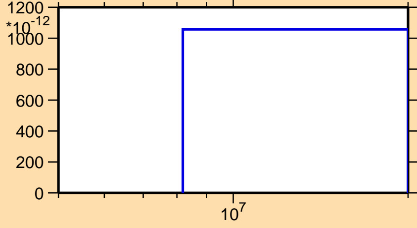
\sigma vs. E for ^{231}\text{Np}(n,nd)
