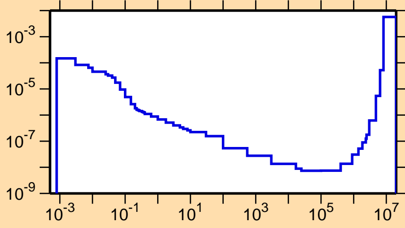
\sigma vs. E for ^{231}\text{Np}(n,\alpha)
