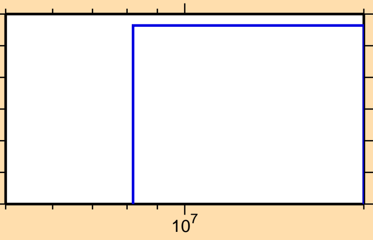
\sigma vs. E for ^{231}\text{Np}(n,3n)
