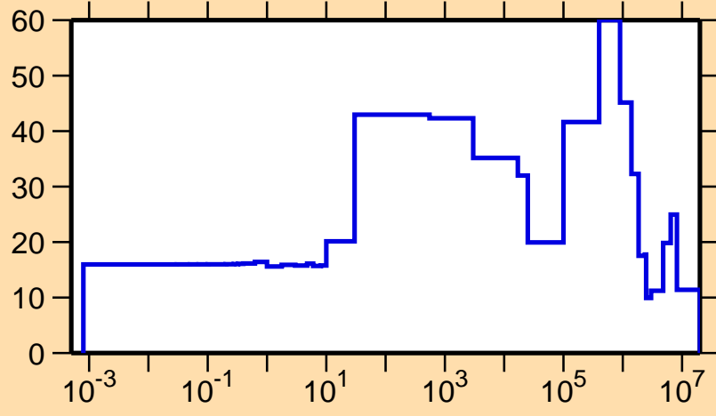
\Delta\sigma/\sigma vs. E for ^{231}\text{Np}(n,el.)
