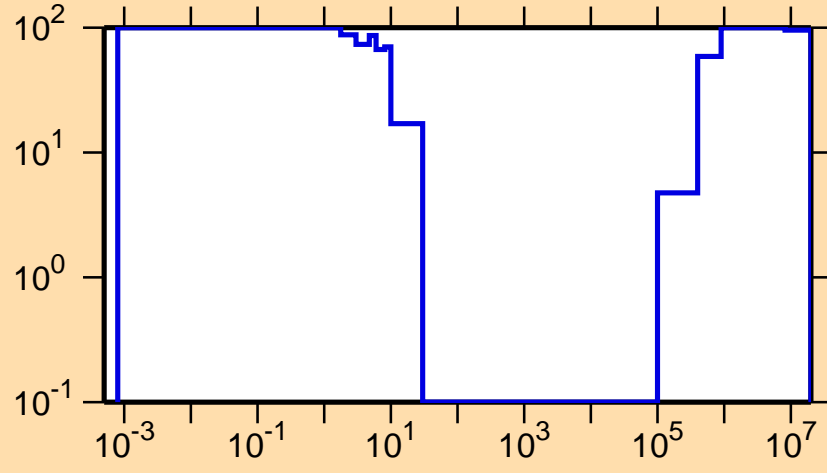
\Delta\sigma/\sigma vs. E for ^{231}\text{Np}(n,p)
