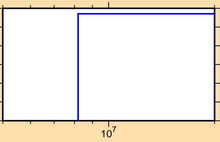
\sigma vs. E for ^{231}\text{Np}(n,\text{He}3)
