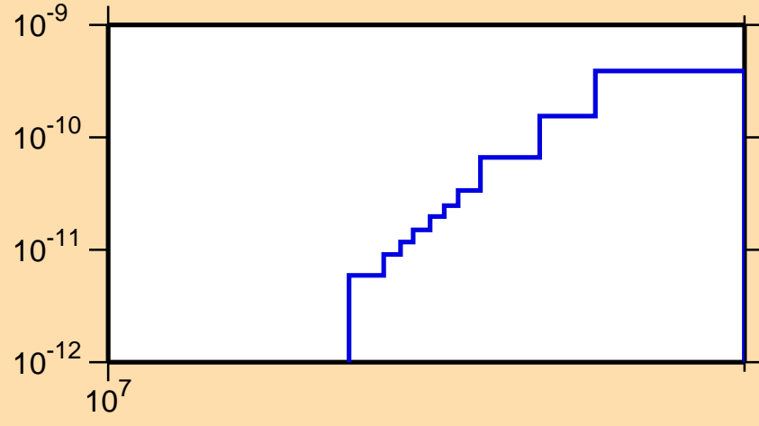
\sigma vs. E for ^{232}\text{Np}(n,p\alpha)
