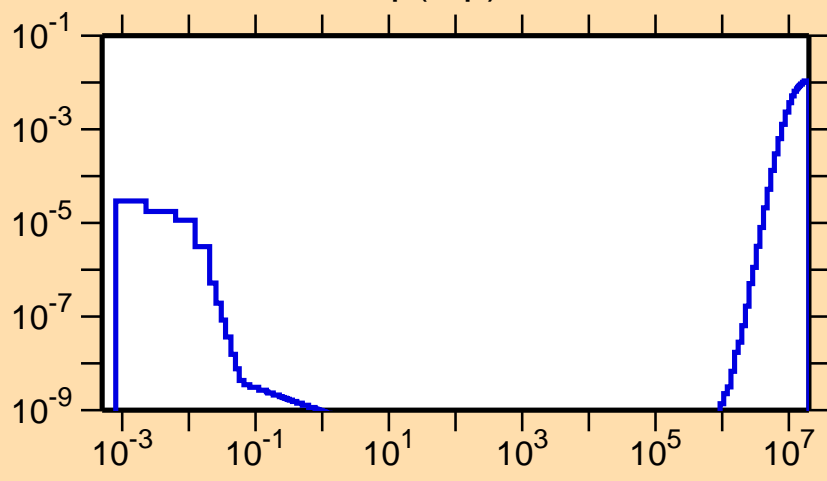
\sigma vs. E for ^{232}\text{Np}(n,p)
