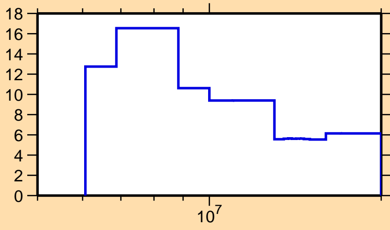
\Delta\sigma/\sigma vs. E for ^{232}\text{Np}(n,\text{tot.})
