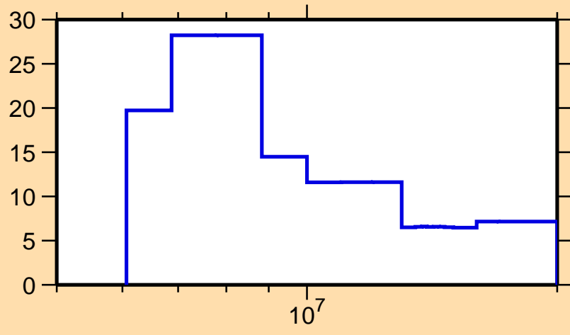
\Delta\sigma/\sigma vs. E for ^{232}\text{Np}(n,\text{el.})
