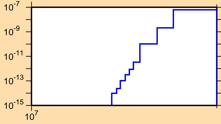
\sigma vs. E for ^{232}\text{Np}(n,nt)
