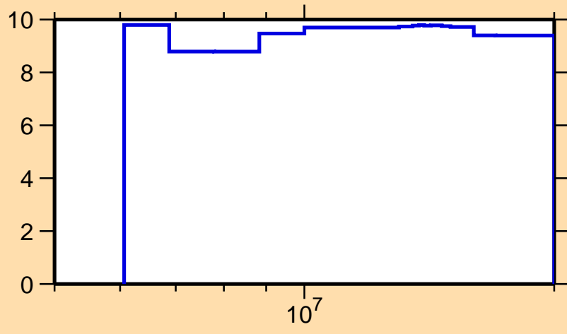
\Delta\sigma/\sigma vs. E for ^{232}\text{Np}(n,\text{nonel.})
