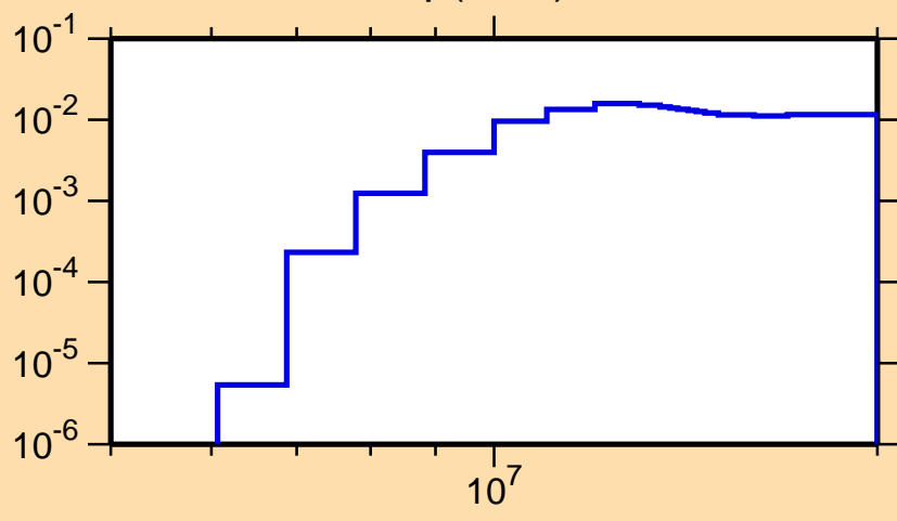
\sigma vs. E for ^{232}\text{Np}(n,2n)
